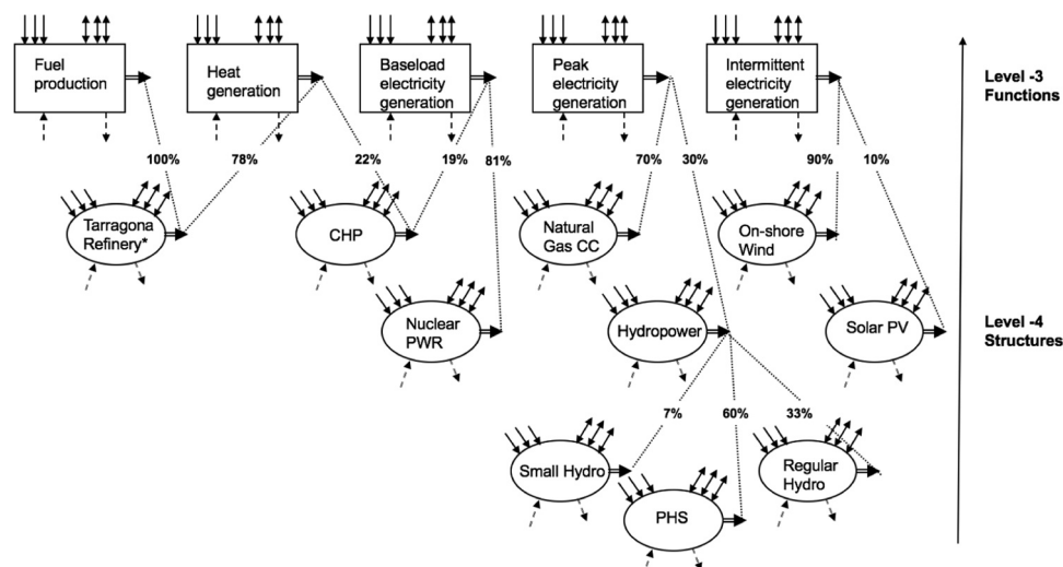
Fig. 4. Functional aggregation of electricity production processors.
