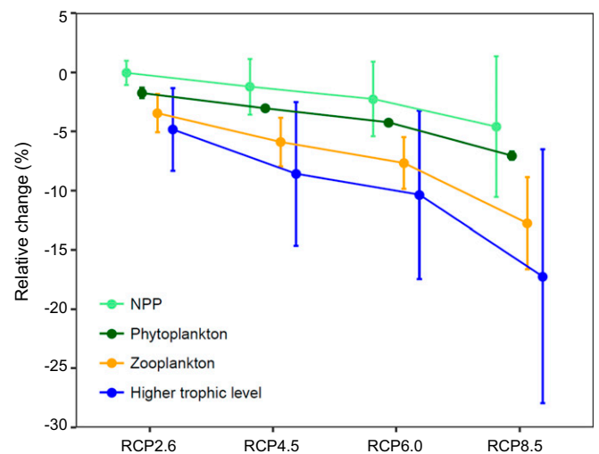
Fig. 3. Trophic amplification of marine biomass declines. Shown is the magnitude of projected mean changes in 2090–2099 relative to 1990–1999 (percent, \pm SD) for NPP, phytoplankton, and zooplankton biomass derived from ESMs ( n = 2 ) and higher trophic levels from MEMs across four RCPs ( n = 10 for RCP2.6 and RCP8.5; n = 8 for RCP4.5 and RCP6.0). All ecosystem models use either NPP or phytoplankton biomass as forcing variables, and some also use zooplankton biomass.
