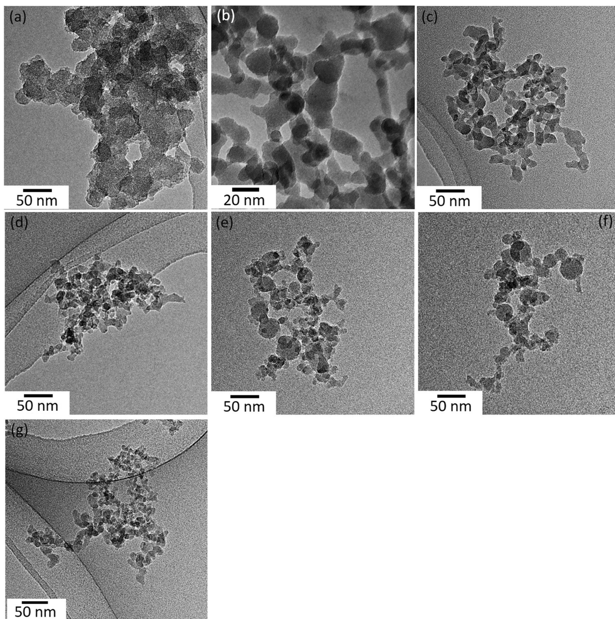
Fig. 1 Bright-field TEM images of (a) WetChem SiO 2 and FSP SiO 2 (b) 5/5, (c) 3/5, (d) 4/5, (e) 9/3 and (f) 11/3, and (g) commercial fumed SiO 2
