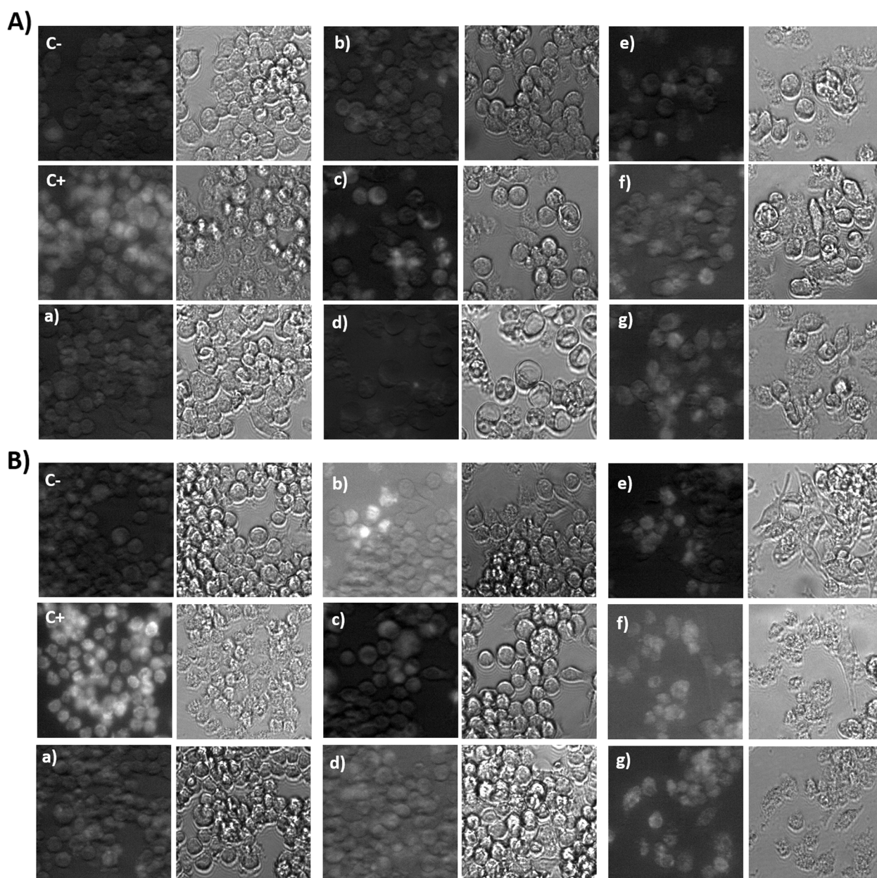
Fig. 5 Confocal images of intracellular ROS generation as a measure of CM-H 2 DCFDA fluorescence in RAW264.7 cells treated with the highest delivered concentration (0.104 \mu\text{g}/\text{cm}^2 ) after 24 h (A) and 72 h (B). Lowercase letters correspond to the different SiO 2 NPs: (a) WetChem SiO 2 and FSP SiO 2 (b) 5/5, (c) 3/5, (d) 4/5, (e) 9/3 and (f) 11/3, and (g) commercial fumed SiO 2 . Controls: (C-) negative control and (C+) positive control treated with H 2 O 2 . Two images were obtained corresponding to green fluorescence channel (left) and transmitted light image (right)
