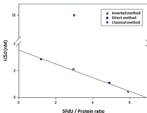
Figure 2. Functional characterization of nanoconjugates. T22-GFP-H6-FdU payload-response trend line representation. Antitumor IC_{50} concentration of each sample was calculated by dose-response curves in MTT cell viability assays upon exposure over CXCR4+ HeLa cells for 48 h. Grey dots represent samples generated by inverted one-pot addition, blue dots represent samples generated by direct-COOH coupling and purple dots represent samples generated by classical two-step protocol. Note that sample from classical two-step protocol doesn't fit in linear regression line.
