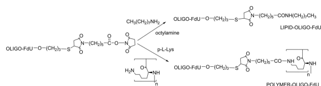
Scheme 2. Schematic representation for the preparation of lipid-oligo-FdU conjugates and polymer-oligo-FdU conjugates using the inverted addition method.
