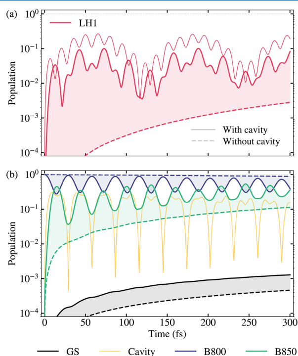
Figure 3. Exciton dynamics for the PSU in Figure 1. (a) LH1 population versus time after the initial excitation of the B800 molecules for the PSU isolated (dashed line) and coupled to an optical cavity with \omega_C = 1.6 eV and g_0 = 9 meV (solid line). The thin solid line plots the LH1 population for an initial excitation of the cavity mode. (b) Temporal evolution of the ground state (black), B800 (blue), and B850 (green) populations with (solid line) and without (dashed line) cavity. The cavity population is shown in the yellow solid line. The differences between populations have been shaded in all cases to highlight the effect of strong coupling.
