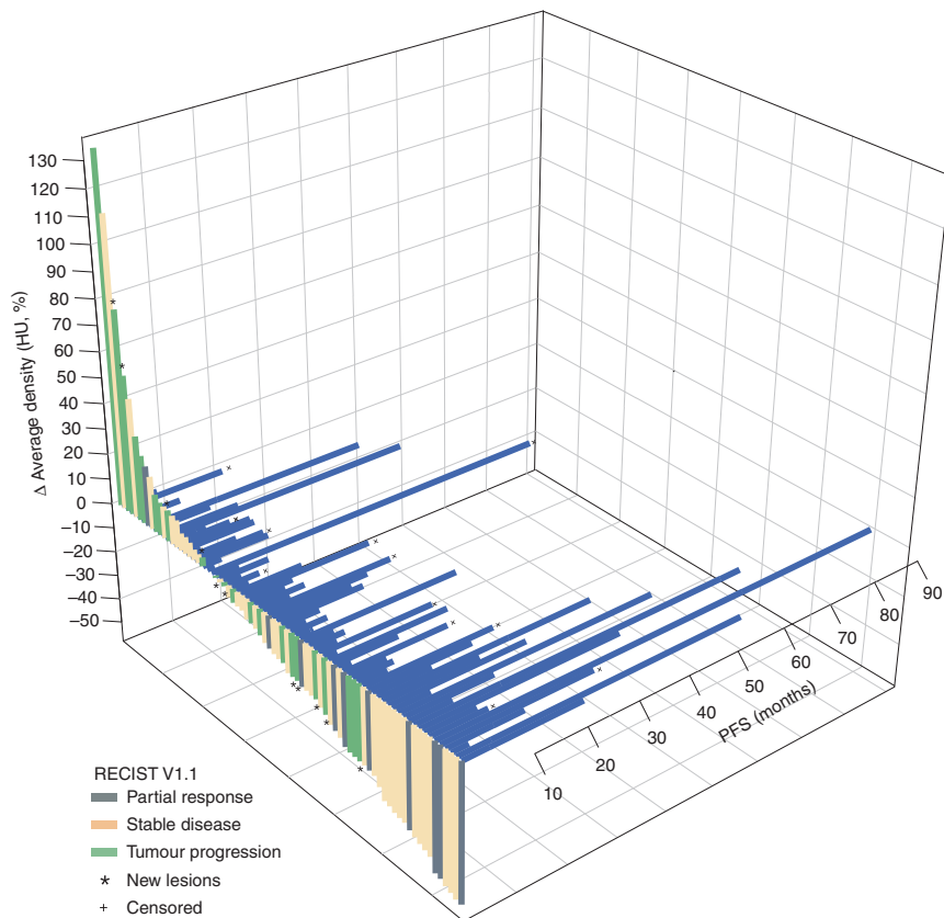
Fig. 4 3D-waterfall plot with the \Delta in the average of HU, RECIST v1.1 and PFS. HU hounsfield units, PFS progression-free survival
