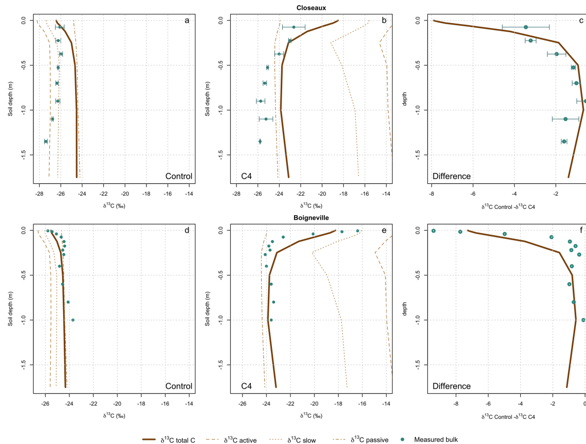
Figure 6. Comparison between simulated and measured soil \delta^{13}\text{C} profiles for the two sites with C3/C4 rotation: Closeaux (a, b, and c) and Boigneville (d, e, and f). The comparisons are for the results from the control plot (under C3 vegetation), the results from the C4 plot and the difference between \delta^{13}\text{C} in the control and C4 plots. The simulated \delta^{13}\text{C} has been decomposed into \delta^{13}\text{C} of the active, slow, and passive pools. Errors bars from data are the observed standard deviation. Please note that for Boigneville only one core was sampled, and consequently we could not calculate the standard deviation.
