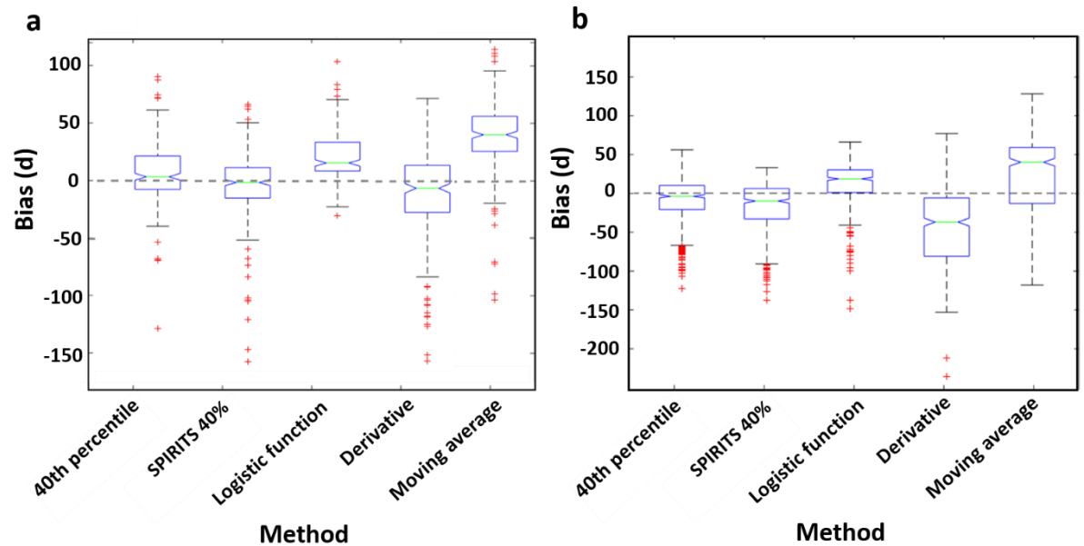
Fig. 8. Boxplots of the bias error for the EoS estimated from LAI V2 minus the ground measurements at the USA-NPN (a) and PEP725 (b) sites. An elongated boxplot indicates a greater dispersion of the average bias in each method.
