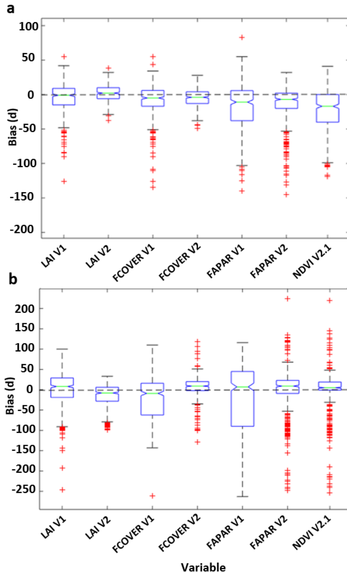
Fig. 4. Boxplots of the bias errors for (a) SoS and (b) EoS estimated from the LAI, FCOVER, FAPAR V1 and V2 and NDVI V2.1 time series minus the PEP725 ground measurements. An elongated boxplot indicates a greater dispersion of the average bias.
