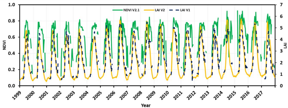
Fig. 2. LAI (V1 and V2) and NDVI (V2.1) time series for the PEP725 site 5449 (50°42'20.49"N, 13°46'59.55"E) representative of birch forest in Europe.
