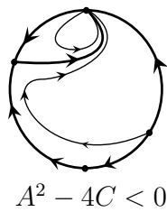
FIGURE 5. Phase portraits in the Poincaré disc of Case (i) when A^2 - 4C < 0 .
