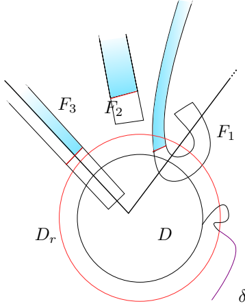
Figure 1: Definition of \overset{B,r}{F} when B is a single basic region. The region B is shown together with the disk D used to define fundamental domains. For simplicity only 3 fundamental domains F_1, F_2, F_3 are shown. The circle of radius r and its preimages inside F_1, F_2, F_3 are in red. Shaded in light blue are the tails of level 1 for the disk D_r corresponding to F_1, F_2, F_3 . The curve \delta_r is in purple.
