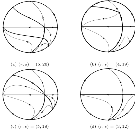
FIGURE 3. Phase Portraits of Case 3.
