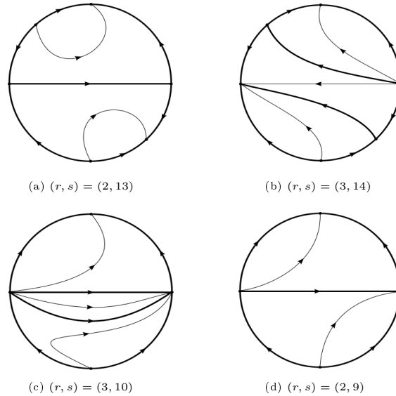
FIGURE 4. Phase Portraits of Case 4.
