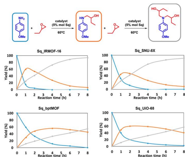
Figure 4. Kinetic plots for the epoxide ring-opening reaction of 4-methoxy aniline (blue) and ethyl epoxide at 60 °C to form the mono-adduct (orange) or bis-adduct (grey) product, in the presence of Sq_IRMOF-16 , Sq_SNU-8X , Sq_UiO-68 or Sq_bptMOF .
