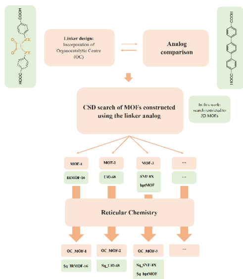
Figure 1. The reticular chemistry-based strategy for rational design of MOF-based catalysts containing organocatalytic centers. CSD: Cambridge Structural Database.
