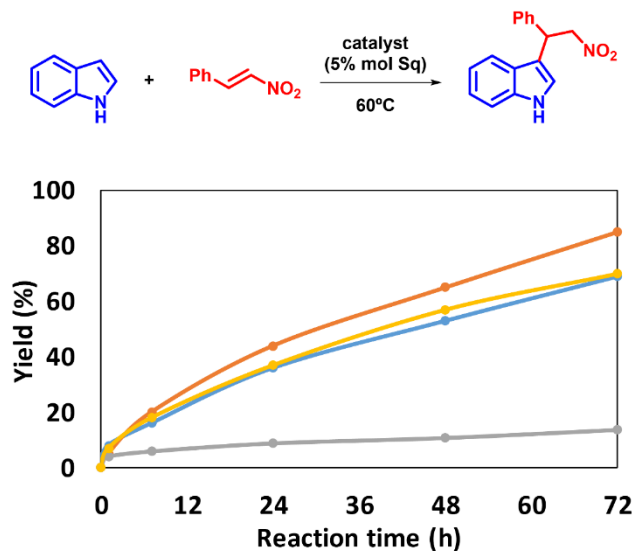
Figure 3. Kinetic plots for the Friedel-Crafts reaction of indole and \beta -nitrostyrene at 60 °C, forming the alkylated product, in the presence of Sq_IRMOF-16 (yellow), Sq_UiO-68 (blue), Sq_SNU-8X (orange) or Sq_bptMOF (grey).
