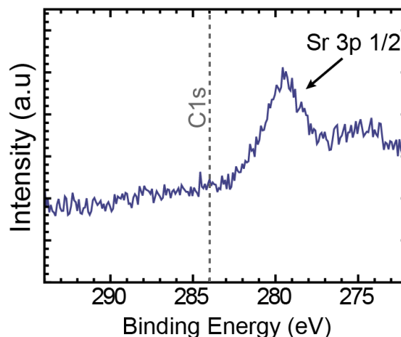
Figure S8. XPS measurements after sample cleaning. Measurements in the range of the carbon 1s excitation post-cleaning procedure reveals no adventitious or carbonaceous contamination on the surface of the samples prior to AP-XAS and AP-XPS measurements.
