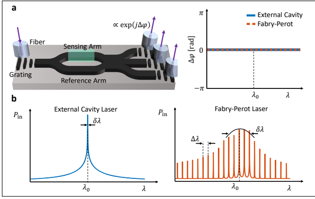
Fig. 1. a Schematic of a coherently read balanced Mach-Zehnder sensor, where the phase difference between the reference and the sensing arm is recovered from three output signals. The wavelength response of such a sensors is completely flat when the optical arm lengths are balanced. b The approximated laser spectra of a narrow linewidth external cavity laser and a Fabry-Perot laser, with center wavelength \lambda_0 , linewidth \delta\lambda , and spectral spacing \Delta\lambda .
