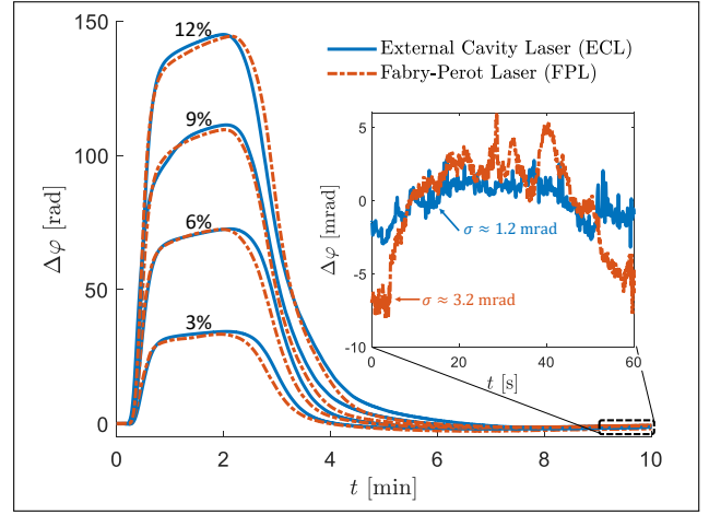
Fig. 2. Bulk sensing using the reference ECL source (continuous blue curve) and the low-cost FPL (dashed orange curve) for 3%, 6%, 9%, and 12% mass percentage sodium chloride injections, respectively, and low input power.
