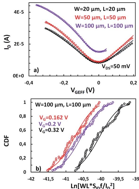
Fig. 2 (a) Drain current I_{\text{D}} vs. top gate voltage overdrive V_{\text{GEFF}} for GFETs with W/L = 20\ \mu\text{m}/20\ \mu\text{m} , 50\ \mu\text{m}/50\ \mu\text{m} and 100\ \mu\text{m}/100\ \mu\text{m} . Markers: measured data, solid lines: model. (b) Cumulative distribution function (CDF) of natural logarithm of normalized LFN \ln(W L S_{I_{\text{D}}} f / I_{\text{D}}^2) , referred to 1 Hz, for GFET with W/L = 100\ \mu\text{m}/100\ \mu\text{m} , shows a log-normal distribution. Markers: extracted CDF, solid lines: theoretical CDF of normal distribution of \ln(W L S_{I_{\text{D}}} f / I_{\text{D}}^2) .
