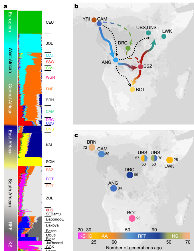
Fig. 2 | Population admixture and genetic ancestry among African populations.
