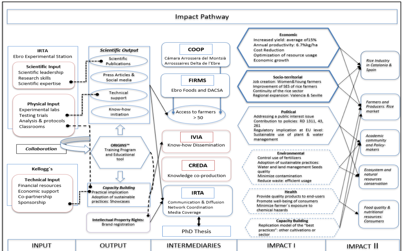
Figure 5. Impact pathway
