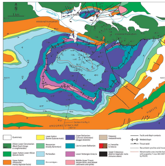
Fig. 12. Geological map of the Tres Croits polygonal weld structure (location in Fig. 2). See cross-section of the structure on S4 in Fig. 4. Map sources: BRGM 1:50,000 scale geological map (Casteras et al., 1970a), Lanusse (1969), Cloix (2017) and original mapping. The central metamorphic area is marked by marble after the Kimmeridgian limestone, with scapolite crystallization and maximum temperatures recorded up to close to 500°C (Villard, 2016; Ducoux, 2017).
