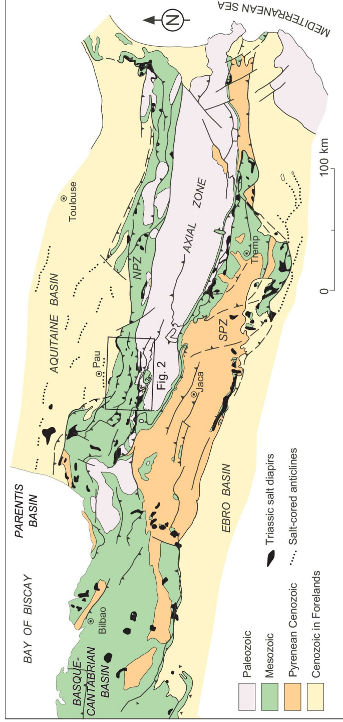
Fig. 1. Structural sketch map of the Pyrenees with location of the main outcrops of Triassic Keuper evaporitic facies. Map modified from Teixell (1996) and Saura et al. (2016). NPZ: North Pyrenean Zone; SPZ: South Pyrenean Zone.
