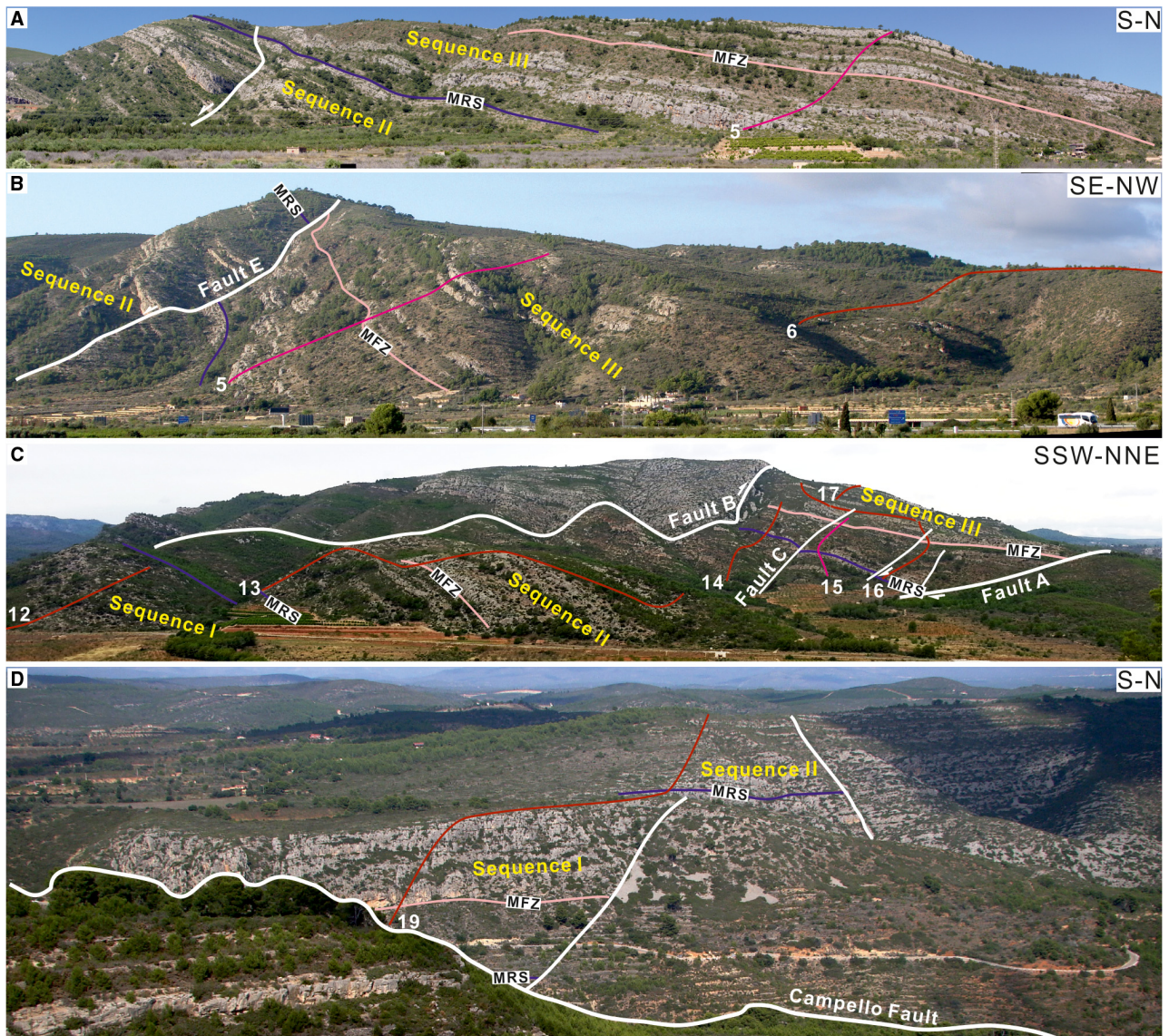
Fig. 4. Panoramic views of the Benassal Formation in: (A) and (B) the north of the Orpesa Range (view is ca 4 km wide); (C) the Ferradura (view is ca 2 km wide); and (D) the Cingle del Morral (view is ca 1.3 km). The traces of field logs are indicated with dark red lines. Sequence stratigraphy surfaces of the Benassal Formation are the maximum regressive surface (MRS) and maximum flooding zone (MFZ). Grey rocks correspond to host limestones, while dolostones present a brownish colour. The numbers in (A) to (D) indicate the corresponding log in Figs 1, 5, 6, 7 and 12.
