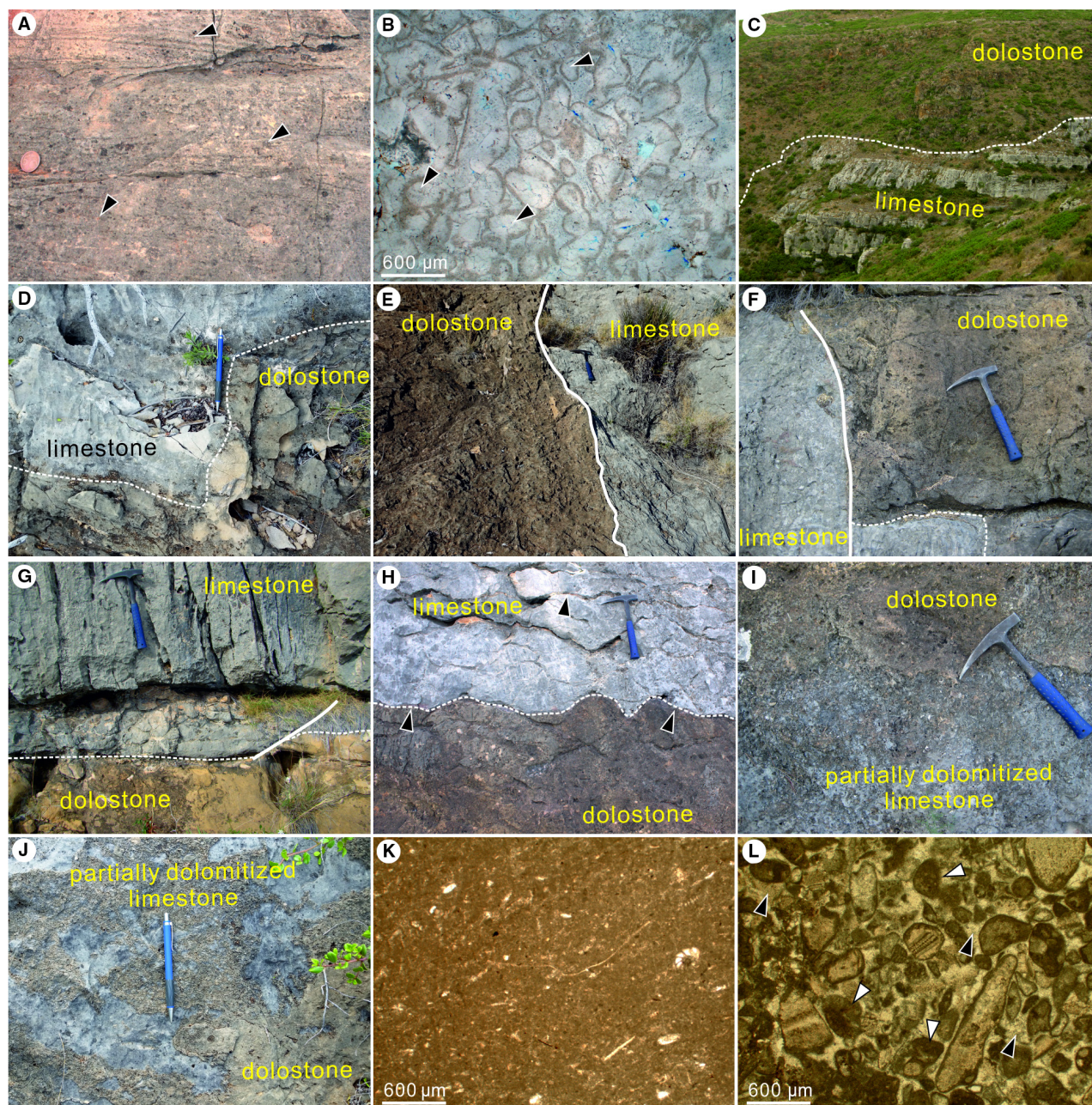
Fig. 9. Main characteristics of limestones and dolostones present in the study area. (A) Close view of a dolostone, most probably dolograinstone, showing well-preserved cross-lamination (black arrows). The coin is 2.1 cm in diameter. (B) Photomicrograph of a replacive dolomite crystal mosaic showing ghosts of the original grain components, which are dominated by peloids (black arrows). Diffused light. (C) and (D) Field view of large-scale (C) and small-scale (D) dolomitization fronts (dashed lines) that are laterally pinching out. Area of view in (C) is ca 180 m high. The pen in (D) is 13.5 cm long. (E) and (F) Close-up view of sharp dolomitization fronts (dashed line) corresponding to an outcrop-scale fault and a fracture (white line), respectively. The hammer is 32 cm long. (G) and (H) Close-up views of sharp dolomitization fronts (dashed line) mainly along bedding planes and wavy stylolites (black arrows), respectively. The hammer is 32 cm long. (I) and (J) Close-up views of transitional (i.e. not sharp) dolomitization fronts, showing partially replaced limestones. Note that most of the replaced limestones corresponds to skeletal components. The hammer in (I) is 32 cm long. The pen in (J) is 13.5 cm long. (K) Photomicrograph of sponge spicule wackestone (LFT9). Plane polarized light. (L) Peloidal (white arrows) grainstone (LFT3) completely cemented by calcite (black arrows). Plane polarized light.
