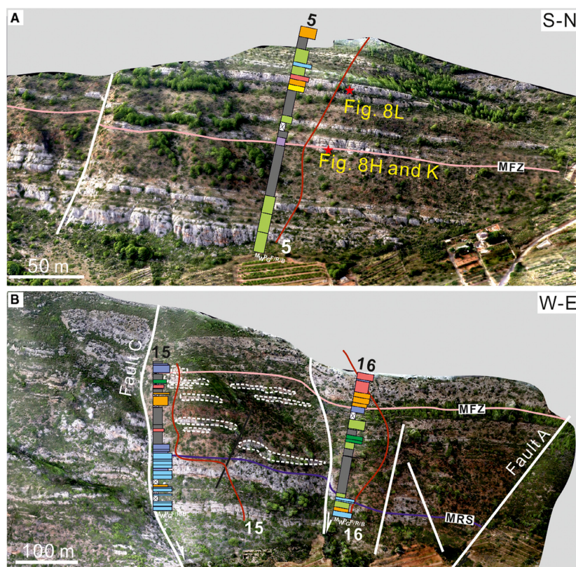
Fig. 11. Photographic view of stratabound dolostones taken from unmanned aerial vehicle (UAV) virtual outcrop models in the north of the Orpesa Range (A) and the Ferradura (B), respectively. Note that stratabound dolostones are significantly more abundant (thicker and with longer extension) and with less limestone stringers in the Orpesa Range when compared with the Ferradura. The outlines of selected limestone stringers within dolostone bodies are indicated with white dash lines in (B). The units represented in the superimposed logs represent those beds found laterally next to the log. See Fig. 5 for lithofacies, texture and sequence stratigraphy legend. Faults are indicated by white lines.
