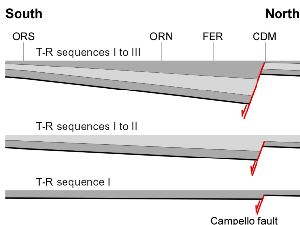
Fig. 13. Sketch of the south to north structure present in the study area illustrating the association of the Campello Fault (red line) with the variation in thickness of sequences I to III. ORS, Orpesa Range-South section; ORN, Orpesa Range-North section; FER, Ferradura section; CDM, Cingle del Morral section; T-R, transgressive–regressive.
