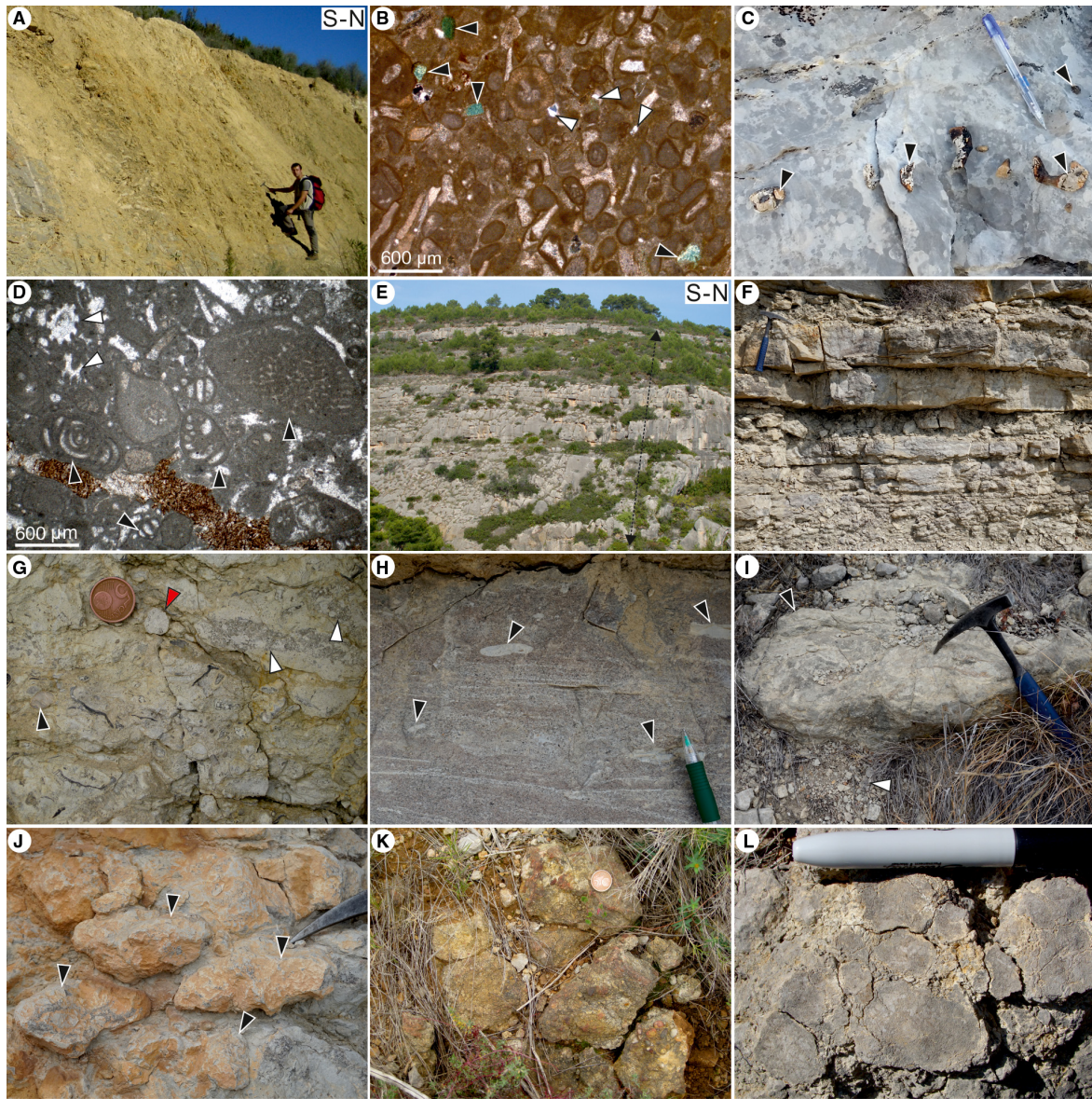
Fig. 8. Field and thin section characteristics of selected lithofacies. (A) Field view of ochre-coloured marls (LFT1) with intercalated peloidal and orbitolinid grainstones (LFT2). The person for scale is 1.85 m tall. (B) Photomicrograph of LFT2 showing abundant glauconite (black arrows) and quartz grains (white arrows). Plane polarized light. (C) Field view of very fine-grained packstones with abundant chert nodules (black arrows) typical of LFT9. Thin section analysis indicate that this lithofacies is rich in sponge spicules and calcispheres. The pen is 13.5 cm long. (D) Photomicrograph of LFT 13 showing the association of foraminifera (black arrows) and dasy-cladales green algae (white arrows). Plane polarized light. (E) Field view of a peloidal grainstones (LFT3) unit from log 18 (arrow length ca 70 m). (F) Field view of LFT14 showing a coarsening and thickening up cycle made of echinoid-sponge-rich packstones to grainstones. The hammer is 32 cm long. (G) Close view of LFT14 showing the poorly sorted character and the presence of echinoids (black arrow), corals (white arrows) and sponges (red arrows). The coin is 2.1 cm in diameter. (H) Close view of LFT14 showing cross-lamination, mud pebbles (black arrows) and mud drapes. The pen is 4 cm long. (I) Field view of LFT15 showing a coral colony in life position (black arrow) embedded in grey marls (white arrow). The hammer is 32 cm long. (J) Field view of LFT15 showing centimetre-sized coral colonies (black arrows) touching each other. The hammer part is 7 cm long. (K) Field view of a conglomerate made of centimetre-sized quartz grains (LFT8). The coin is 1.6 cm in diameter. (L) Close view of mud cracks appearing at the top of shallowing up cycles. The pen is 10 cm long.
