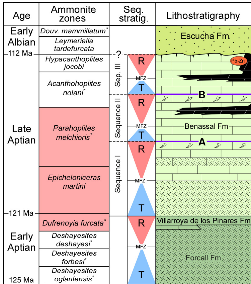
Fig. 2. Chronostratigraphy, biostratigraphy and lithostratigraphy chart showing the sequence stratigraphy framework of the Benassal Formation in the study area as well as the location of dolostones (black colour) (modified from Martín-Martín et al. , 2015). Ammonite biozones identified in the study area are shaded in red. Dashed lines in transgressive–regressive (T–R) sequences indicate lack of absolute dating, and purple lines denote the maximum regressive surfaces (MRS) of sequences I (A) and II (B) (see blue lines in Fig. 1 for their trace on the geological map). MFZ, maximum flooding zone; R, regressive system tract; T, transgressive system tract. Bottom and top boundaries of lithological formations after Bover-Arnal et al. , 2016.
