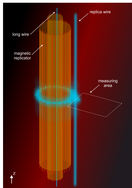
FIG. 1. A long wire is surrounded by a magnetic replicator generating a replica of the wire outside it.
