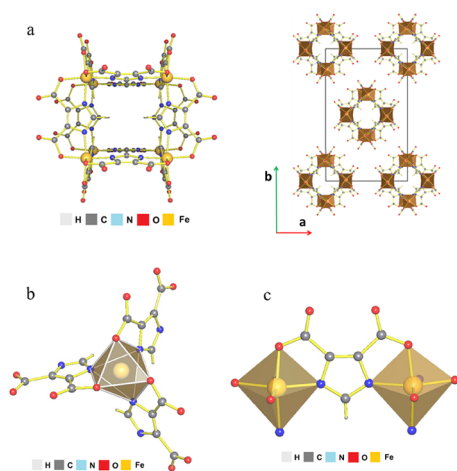
Figure 1. (a) Molecular structure of 1 and view of the packing through the c axis. (b) Coordination environment of Fe III centers in 1 and (c) \mu -1 \kappa^2 N,O:2 \kappa^2 N',O''' bis-chelating bridge mode of IDC 3- .
