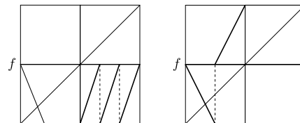
Figure 25 Examples of maps with a = -1 , d = 0 , and bc = 0
