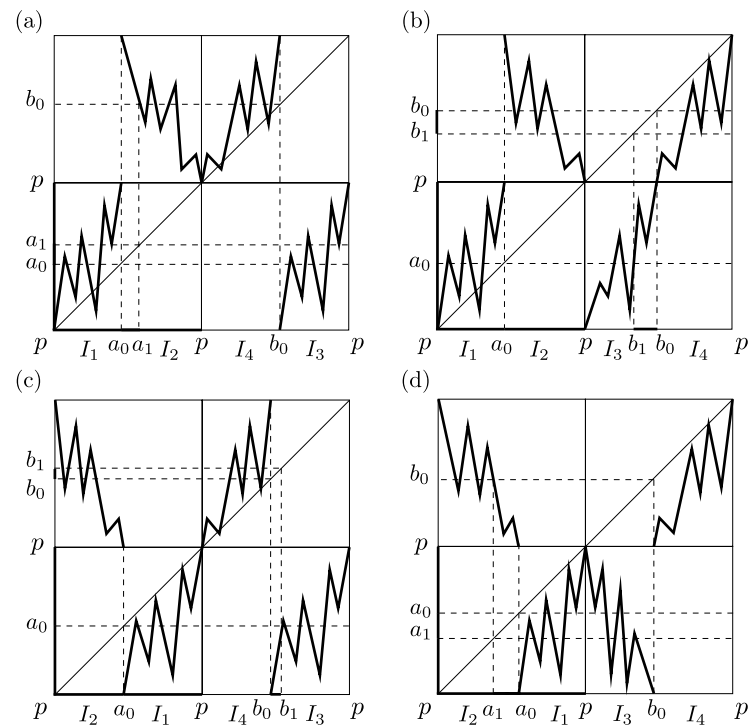
Figure 14 Examples of maps with \{a, d\} \subset \{-1, 0, 1\} , |a| + |d| = 2 , b = 1 , and c = -1
