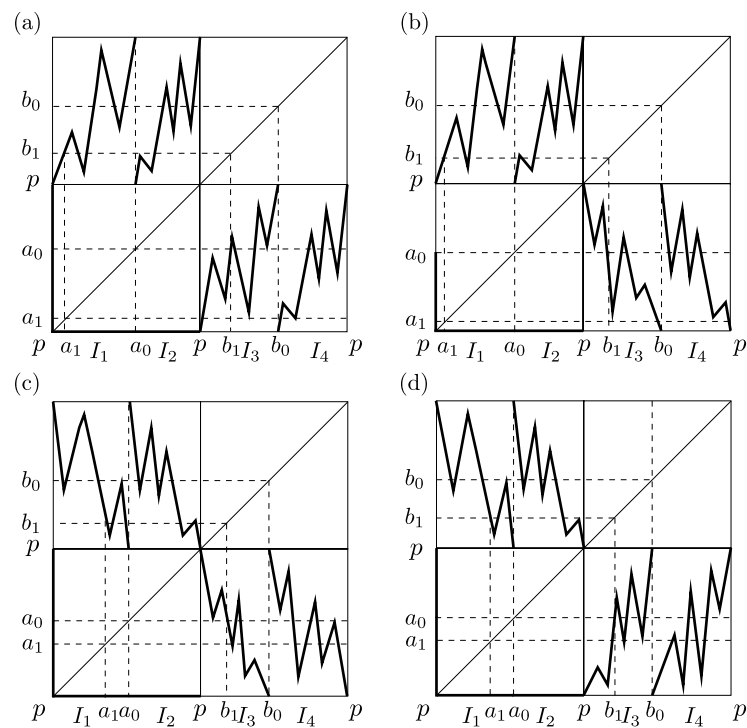
Figure 35 Examples of maps with a = d = 0 and |b| = |c| = 2
