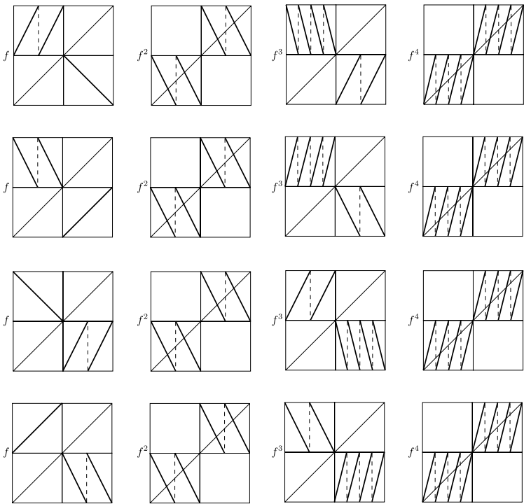
Figure 30 Examples of maps with a = d = 0 , bc = -2 , and 4 \notin \text{Per}(f)
