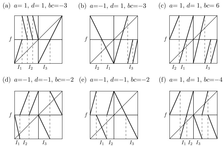
Figure 7 Examples of maps with \{a, d\} \subset \{-1, 0, 1\} , |a| + |d| = 2 , and |bc| > 1
