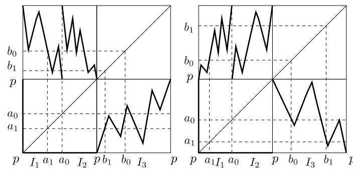
Figure 31 Examples of maps with \sigma = d = 0 and bc = -2
