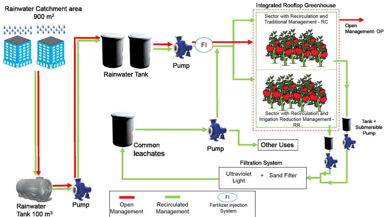
Fig. 2. The three irrigation schemes, including auxiliary equipment. OP management (red line), recirculated management (green line).
