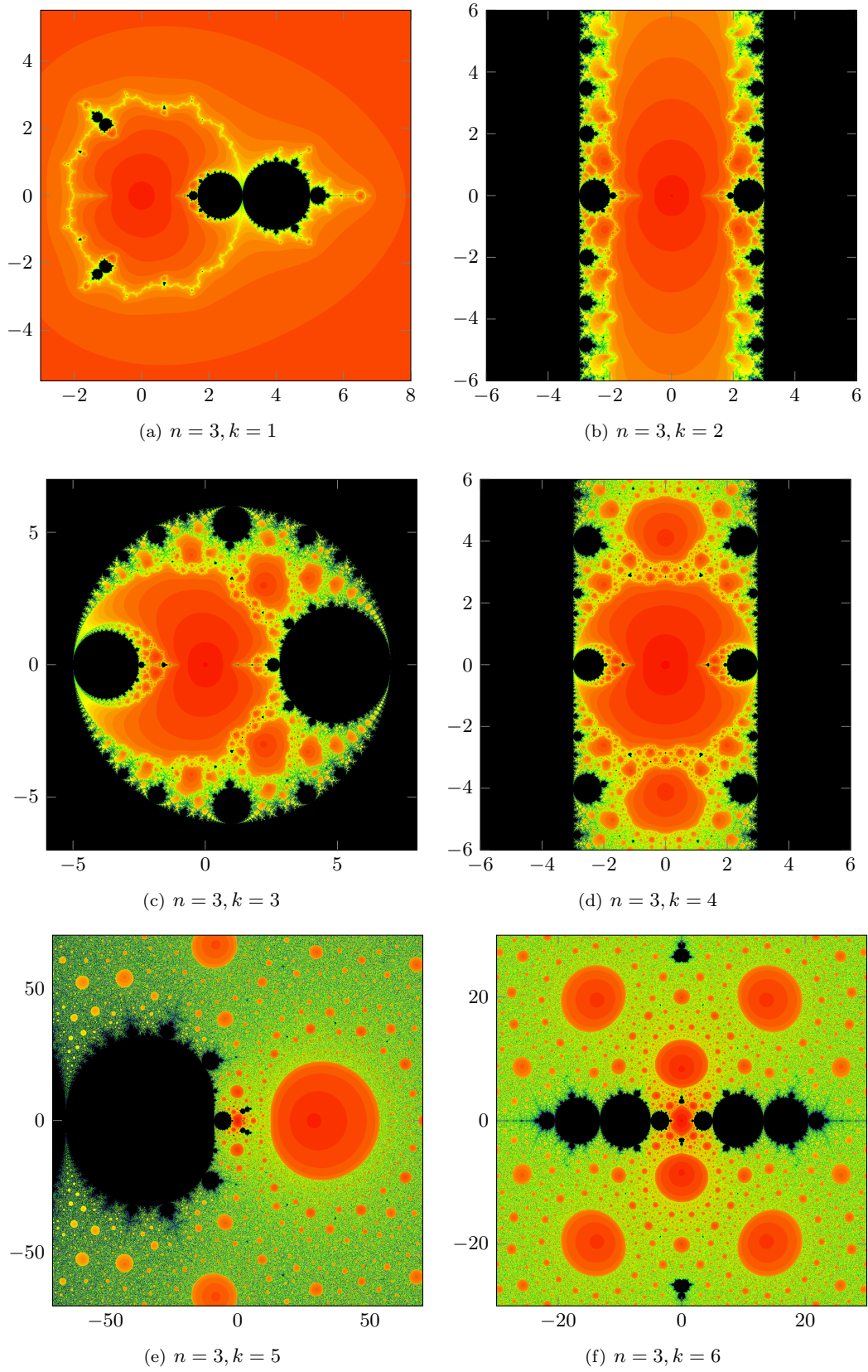
FIGURE 7. Parameter planes of O_{a,n,k}(z) for n=3 .
