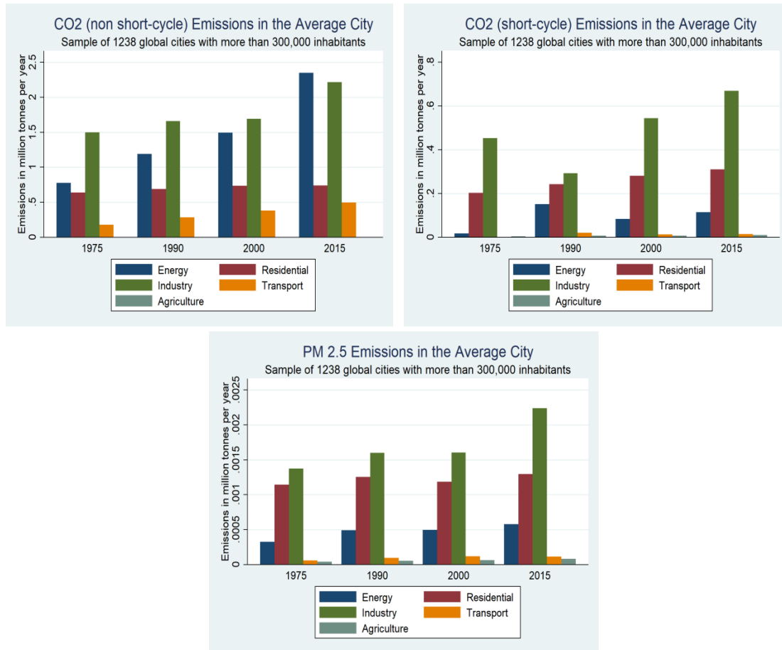
Figure A.2 Time Trends of Different Emission Types
