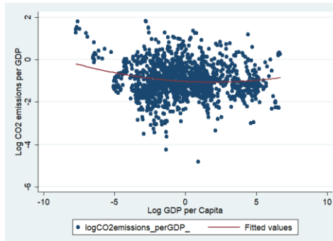
(B) Log GDP pc and log CO2 emissions per GDP
