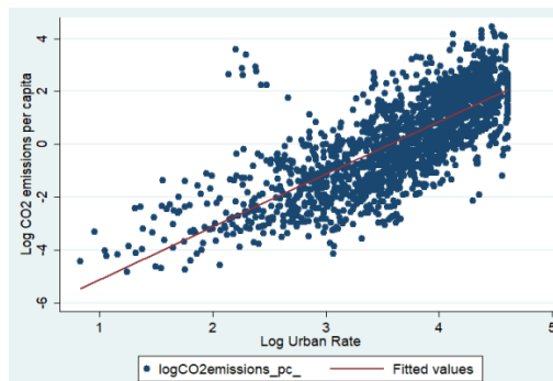
(E) Log urban rate and log CO2 emissions pc
