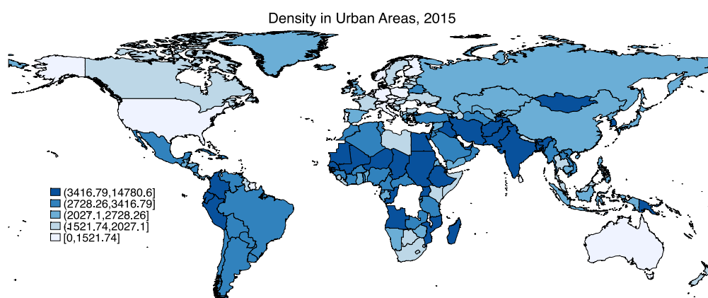
Figure 3: Density in urban areas, 2015
