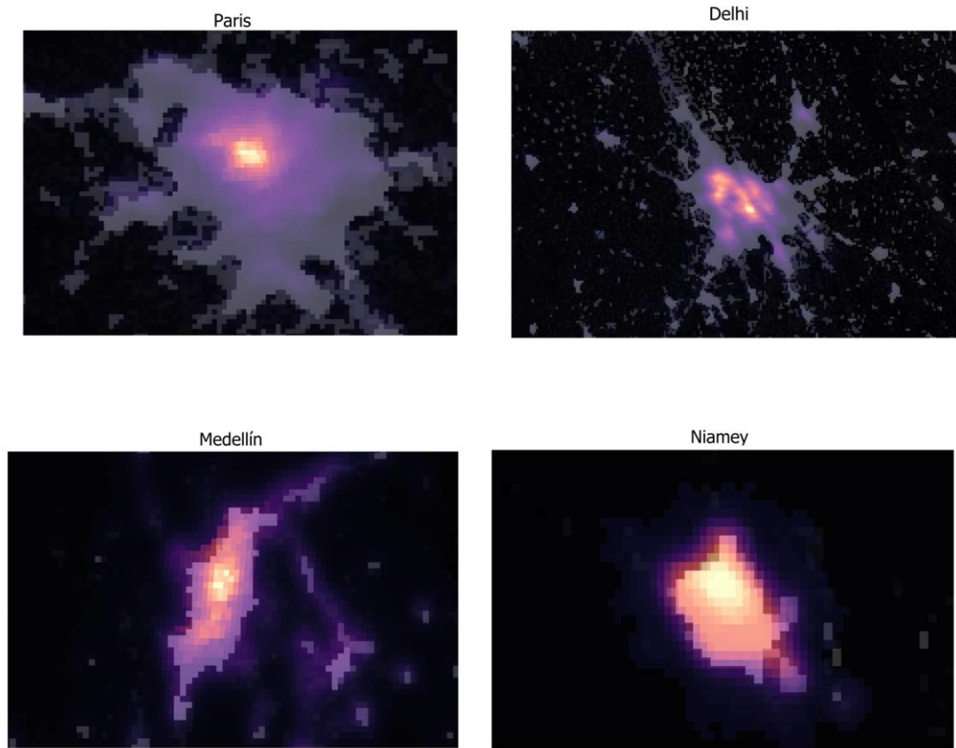
Figures A.1: Spatial Structure of Four Different Cities
