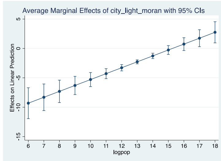
Figure B.1: Marginal effects of structure depending on city size
