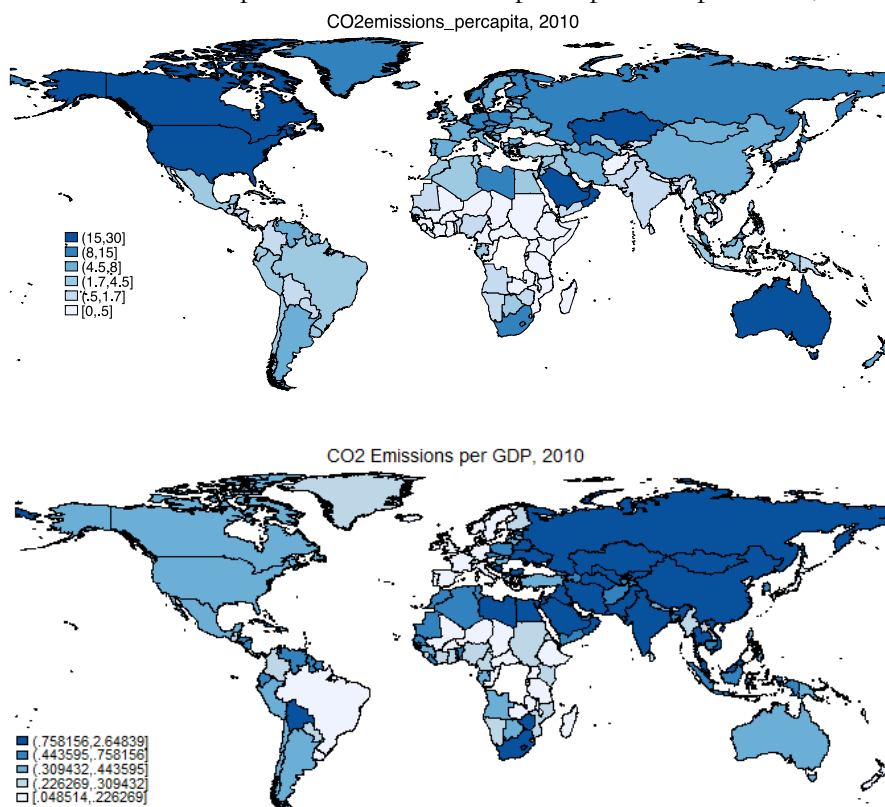
Figure C.1.a and C.1.b: Maps of CO2 Emissions per capita and per GDP, 2010
