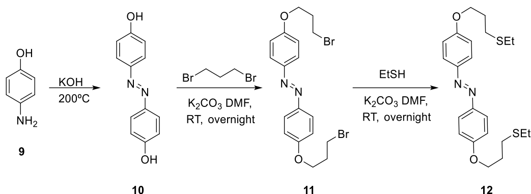
Scheme 2. Synthetic strategy for ligand 12 .
