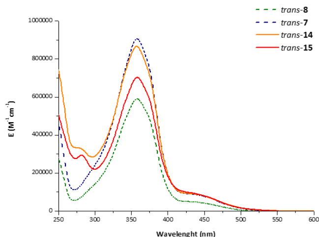
Figure 2. Absorption spectra of compounds 7 , 8 , 14 and 15 in ACN. Measurements were carried out at low concentrations ( \sim 10^{-5} M) to minimize aggregation processes.
