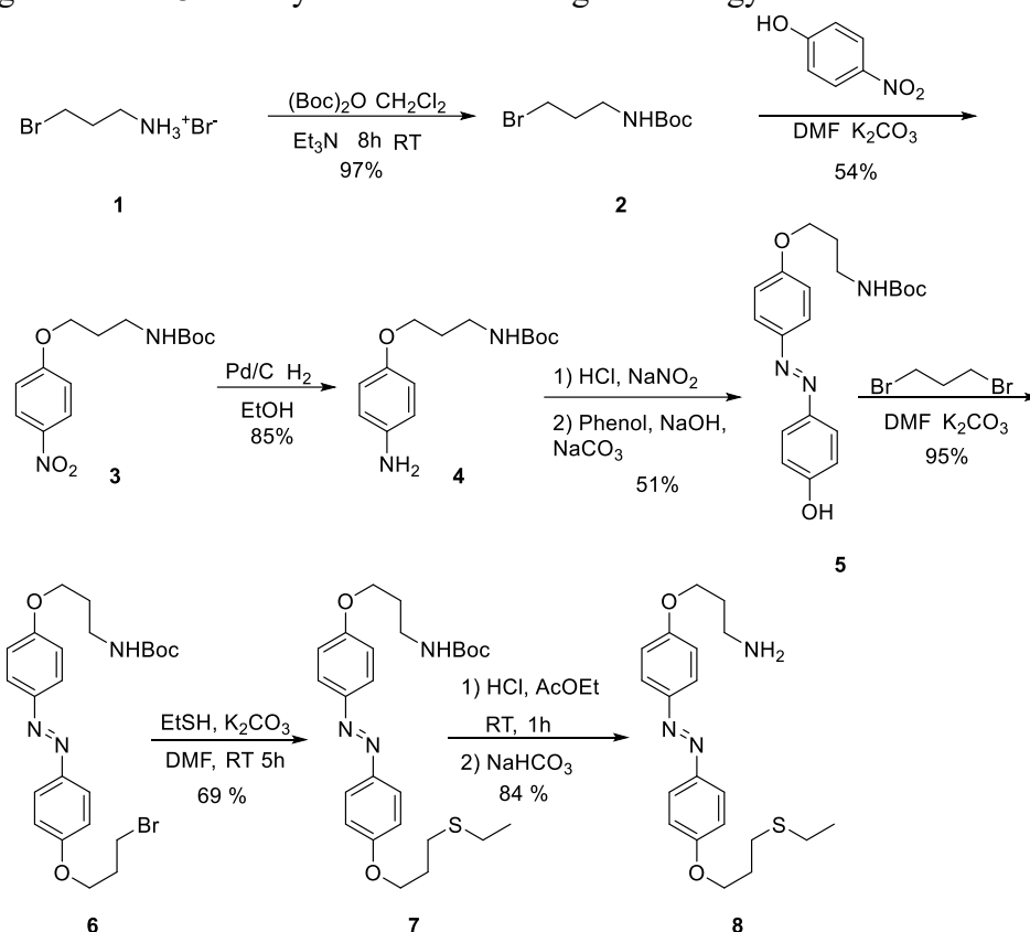
Scheme 1. Synthetic strategy for ligands 7 and 8 .
