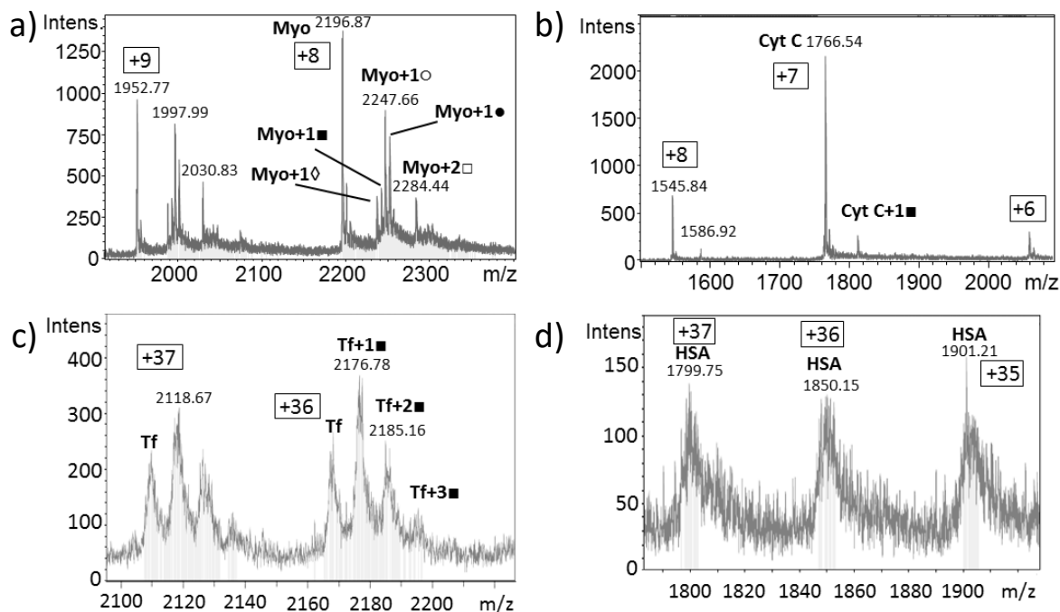
Figure 9. Mass spectra of 14 recorded after incubation for 24 h at 37 °C with a) myoglobin (Myo) and b) cytochrome C (Cyt C) at a 1:10 (protein:Pt) molar ratios, c) transferrin (Tf) at a 1:5 (protein:Pt) molar ratios and d) human serum albumin (HSA) at a 1:1 (protein:Pt) molar ratios. The numbers preceded by the “+” symbol in the boxes denote the charge state of the peaks. The notation “+ n\circ ”, where n is a number after the name of the protein, denotes a mass increase corresponding to the addition of “ n ” molecules of complex 14 to the protein after the elimination of chloride and azobenzene ( 8 ) ligands, and the coordination of one dmso (738.25-409.01+78.1 mass units at the corresponding charge state); the notation “+ n\blacksquare ” indicates a mass increase corresponding to the addition of “ n ” molecules of complex 14 after elimination of chloride and azobenzene ( 8 ) ligands (738.25-409.01 mass units at the corresponding charge state); the notation “+ n\Diamond ” indicates a mass increase corresponding to the addition of “ n ” molecules of complex 14 after elimination of azobenzene ( 8 ) ligand (738.25-373.51 mass units at the corresponding charge state); the notation “+ n\bullet ” indicates a mass increase corresponding to the addition of “ n ” molecules of complex 14 after elimination of azobenzene ( 8 ) ligand, and the coordination of one dmso (738.25-373.51+78.1 mass units at the corresponding charge state); the notation “+ n\Box ” indicates a mass increase corresponding to the addition of “ n ” molecules of complex 14 after elimination of chloride ligand (738.25-35.5 mass units at the corresponding charge state).
