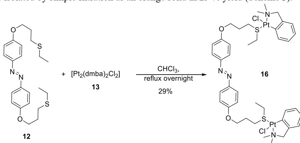
Scheme 5. Synthesis of dinuclear complex 16 from azobenzene 12 and precursor 13 .
