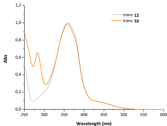
Figure 5. Normalized absorption spectra of compounds 12 and 16 in \text{CH}_2\text{Cl}_2 . Measurements were carried out at low concentrations to minimize aggregation processes ( \sim 10^{-5} M).
