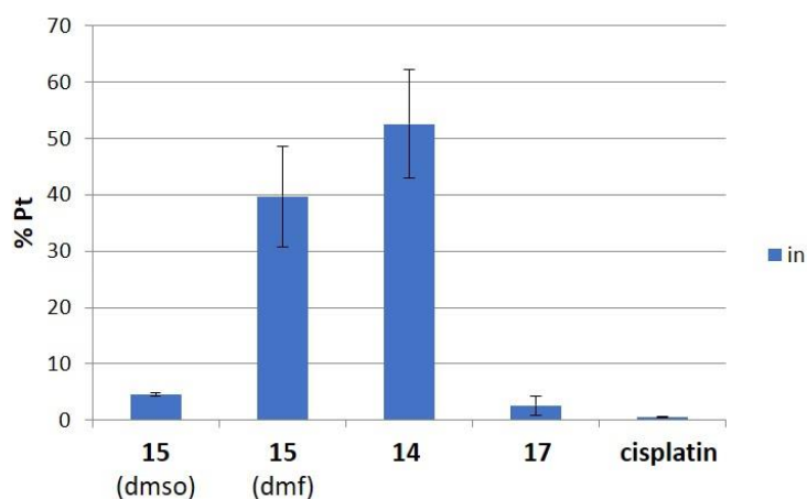
Figure 7. Percentage of Pt(II) inside HeLa cells after uptake studies with 10 µM of complex exposure for 3 h. Samples were analyzed by ICP-MS after being digested with ultra-pure concentrated nitric acid. The stock solution was also measured and set as the 100 % of the amount of platinum used, together with the amount “external-platinum”. Complexes 14 and 17 are containing dmso as solvent.
