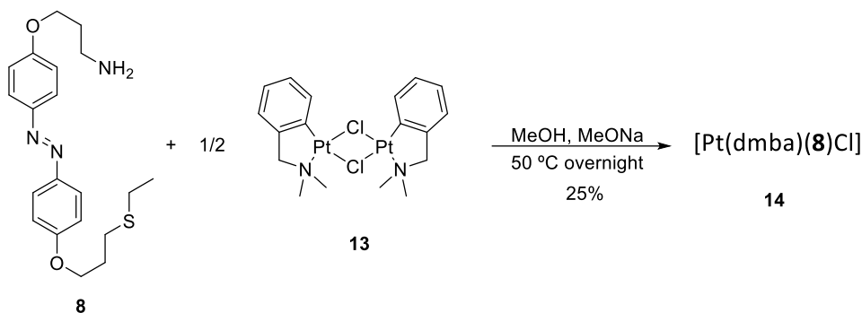
Scheme 3. Synthesis of [Pt(dmmba)( 8 )Cl], 14 .
