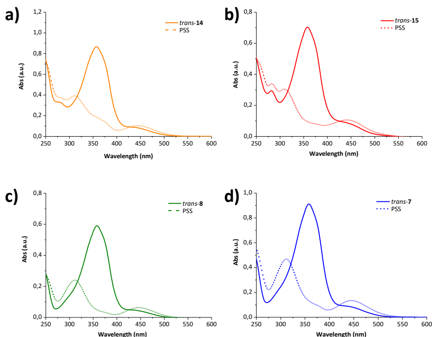
Figure 3. Absorption spectra in ACN of the trans -isomer and the PSS for complexes: a) 14 , b) 15 , and their corresponding ligands: c) 8 and d) 7 .
