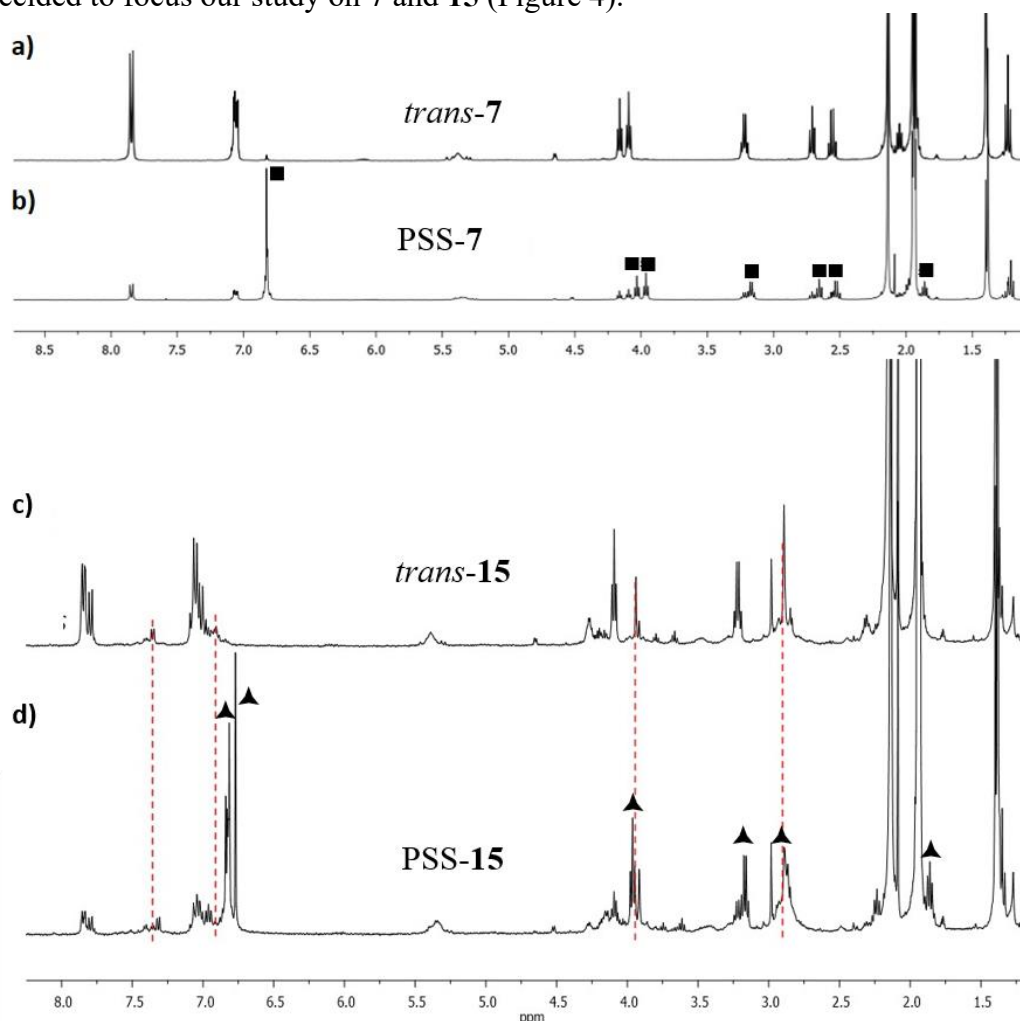
Figure 4. a) 1 H-NMR spectrum of ligand trans - 7 in CD 3 CN, 298 K. b) 1 H-NMR spectrum after irradiation of trans - 7 at 365 nm (PSS- 7 ), signals corresponding to cis - 7 and trans - 7 isomers are visible. c) 1 H-NMR spectrum of ligand trans - 15 in CD 3 CN, 298 K. d) 1 H-NMR spectrum in CD 3 CN, 298 K of complex 15 after irradiation at 365 nm (PSS- 15 ). (■ = Signals assigned to the cis - 7 isomer. ▲ = signals assigned to cis - 15 ).
