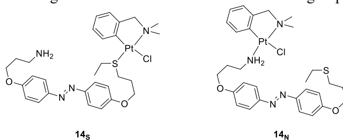
Figure 1. Proposed structures for both isomers of 14 . According to similar examples in literature, S,N-trans configuration has been tentatively assigned for Pt complexes in this work [23]. By analogy, 14 N has been also proposed as N,N-trans .
