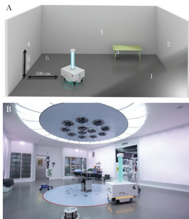
Figure 1. Schematic representation of the autonomous sanitary sterilization ultraviolet machine (ASSUM) UV-C device. A , Position of tested desiccated severe acute respiratory syndrome coronavirus 2 (SARS-CoV-2) samples and chemical indicators in the experimental box. Black numbers indicate positions of samples at 100 cm height on the 4 room walls and sample 5 located under the edge of a table. Sample 6 was located on the floor in a corner of the room. B , Simulation of ASSUM running in an operating room of a hospital.
