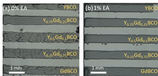
Figure 2. OM images of the as-deposited combinatorial samples showing the stripe morphology for inks with a 50/50 ratio of PPA/BuOH, and containing (a) 0% and (b) 1% of EA. Drop pitches of 50 \mu m and 95 \mu m along the x - and y -directions were employed.
