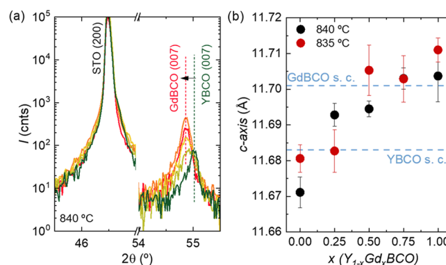
Figure 7. (a) High-resolution XRD diffractograms of a sample annealed at 5^\circ C/s , 840^\circ C for 2 min and a PO_2 of 1 mbar, depicting the (200) STO substrate peak position and the (007) peak for each Y_{1-x}Gd_xBCO composition. (b) Evolution of the c -axis parameter for Y_{1-x}Gd_xBCO samples annealed at 5^\circ C/s up to 835^\circ C and 840^\circ C for 2 min and a PO_2 of 1 mbar. The (001) REBCO peaks and associated shifts, as shown in (a), are translated into lattice parameter variations using the Nelson-Riley criteria (Figure S4). Blue lines indicate the theoretical values from the ICSD database, 11.701 and 11.683 Å for the optimally doped GdBCO and YBCO. Error bars are obtained from the Nelson-Riley linear regression.
