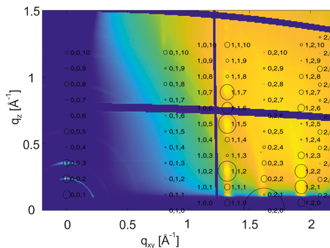
Figure 3. Reciprocal space map of a thermal-gradient crystallized thin film (translation velocity 2.5 \text{ μm/sec} ) together with the indexation of the diffraction pattern based on the known bulk structure of the molecule Ph-BTBT-10. For indexation, only the strongest Bragg peaks are depicted by circles, where the center and areas of the circles give the peak positions and peak intensities, respectively.
