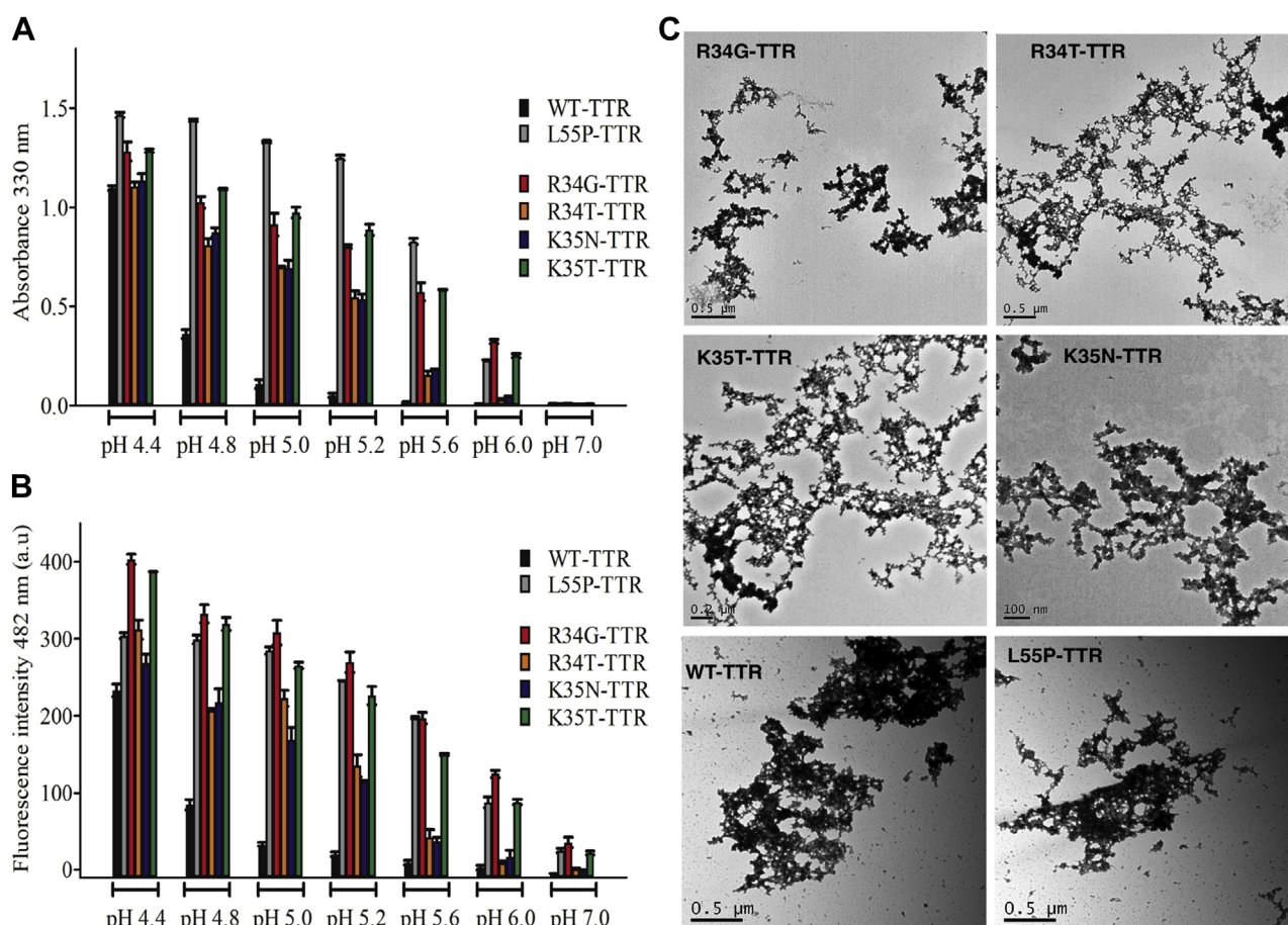
Figure 1. pH dependence on aggregation propensity and amyloid protofibril formation of TTR disease associated variants. 3.5 μM of WT and pathogenic TTR variants were incubated in 100 mM Tris.HCl, 50 mM MES, 50 mM sodium acetate, and 0.1 M KCl at different pHs (ranging from 4.4 to 7.0), for 72 h at 37 °C prior measurements. The amount of protofibril formation as a function of pH was determined by measuring the suspension turbidity at 330 nm (A) and the increase in fluorescence intensity at 482 nm in ThT-binding assays (B). Each experiment was performed in triplicates. C, TEM images of the aggregates of TTR variants, formed at pH 4.4 at 37 °C. Scale bars values are indicated.
