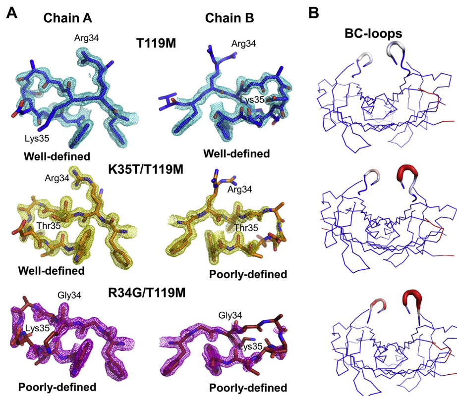
Figure 6. Structural features of T119M, R34G/T119M, and K35T/T119M TTRs. A , stick representation showing the BC-loop regions of TTR dimers with electro densities maps countered at 1.5\sigma . B , Putty cartoon of B-factor variation on the A/B dimers, colored from low to high (blue to red). Side chains of mutated residues are depicted as sticks. Rendered using PyMOL.
