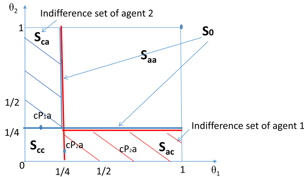
Fig. 4. Partition of S in Example 5.
