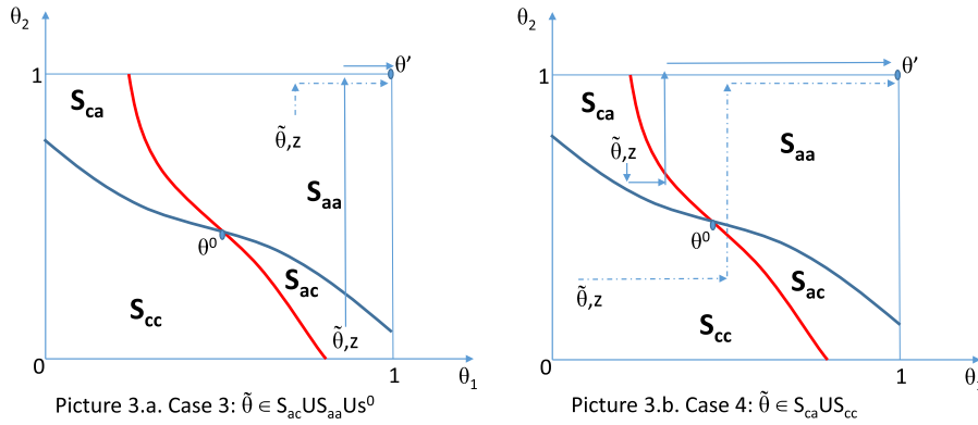
Fig. 3. Changes of agents' types in Cases 3 and 4, proof of Proposition 8.
