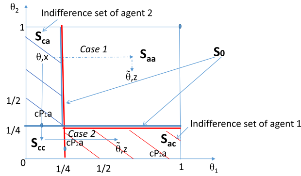
Fig. 5. Changes of agents' types, proof of Proposition 9.
