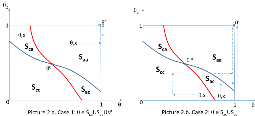
Fig. 2. Changes of agents' types in Cases 1 and 2, proof of Proposition 8.
