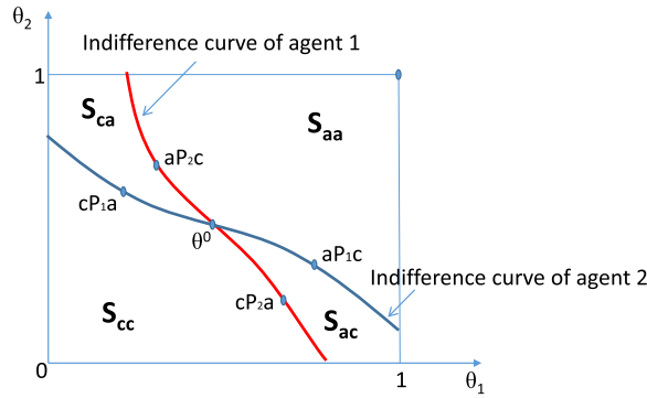
Fig. 1. Examples of the partition of S in Example 4.
