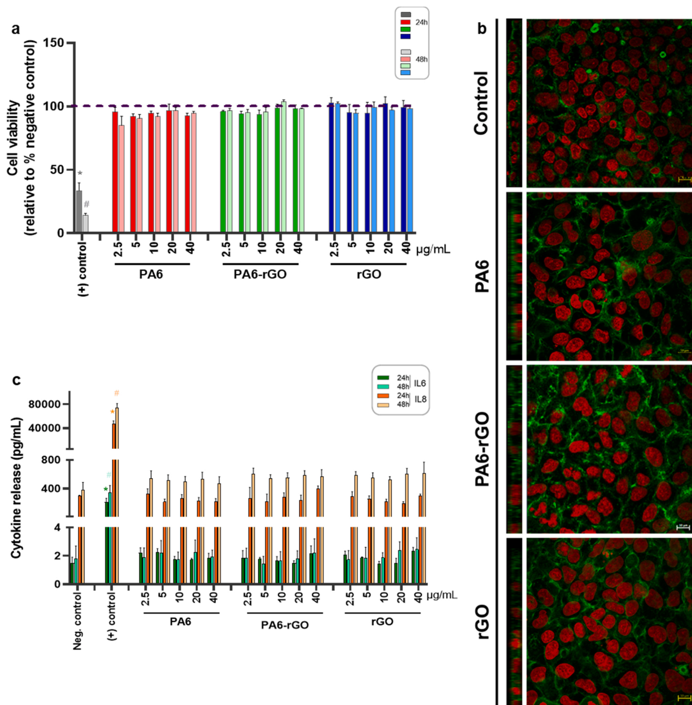
Fig. 3. (a) Cell viability of A549 epithelial cells, measured by the MTS assay after 24 h and 48 h treatment with rGO and the abraded particles from neat PA6 and PA6-rGO composites. 1000 μM CdSO 4 was used as a positive control. (b) Confocal LSM images of A549 cells after exposure to the tested materials (scale bars: 10 μm). The green color shows F-actin (cytoskeleton), red color shows DNA (cell nuclei). (c) Pro-inflammatory response of A549 epithelial cells after treatment with the tested materials. Concentrations of IL-6 and IL-8 were measured after 24 h and 48 h of materials exposure. One μg/mL TNF-α was used as the positive control. The results are shown as mean ± standard error of the mean (SEM) from at least three independent experiments. * indicates statistical significance compared to the negative control at 24 h of exposure ( p < 0.05 ). # shows a statistically significant response ( p < 0.05 ) at 48 h of material exposure.
