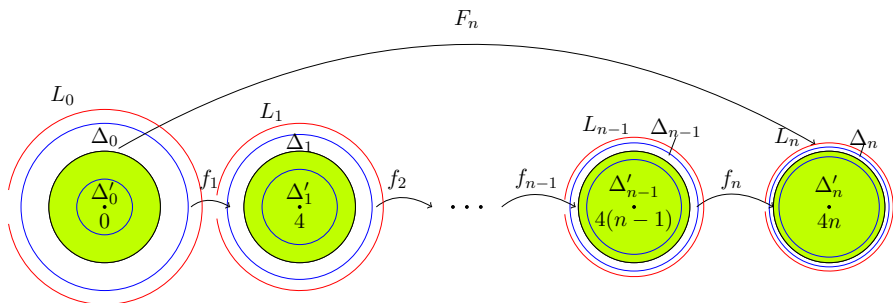
Fig. 6 Sketch of the setup of Theorem 5.3. In green, the disks D_n centred at 4n . In blue, the boundaries of the disks of radii r_n and R_n in between which lie the boundaries of the wandering domains. In red, the curves L_n introduced in the proof (color figure online)
