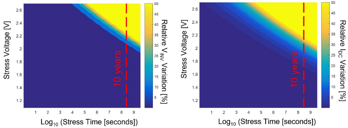
Figure 6: Colored map of the V_{INV} (Left) and I_{DC} (Right) relative degradation as a function of the stress voltage and stress time, evaluated using the equations indicated in figure 5 and parameters in table 1. The red dashed line corresponds to the expected 10 years lifetime.
