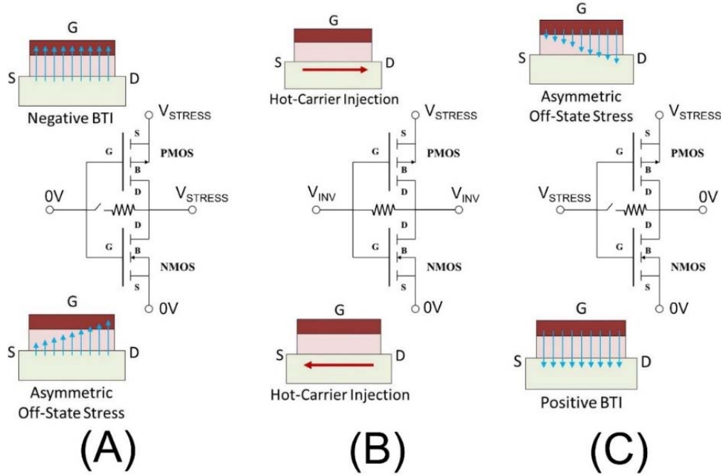
Figure 1. CMOS inverter voltage configuration and active aging mechanisms at (A) low input, (B) inversion point, and (C) high input. The vertical electric field at the gate dielectric during BTI and OFF-State aging (blue arrows) and the currents for HCI (red arrows), for the different inverter stress conditions, are also depicted.
