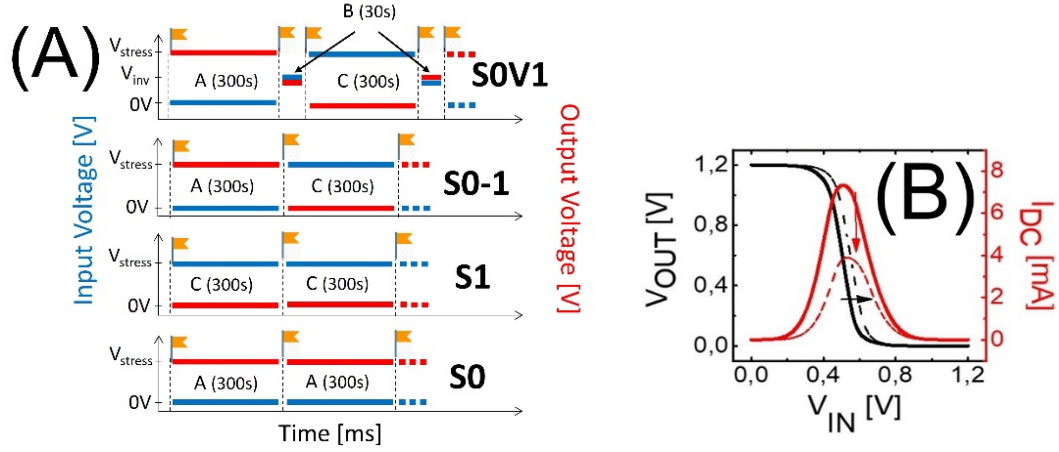
Figure 2. (A) Applied input (blue) and output (red) voltages for each stress sequence. V_{STRESS} was varied to evaluate the voltage dependence of the degradation. Labels indicate the stress voltage configurations of the transistors: (S0V1) alternation of low and high inputs, with and intermediate 30 seconds stage where input and output voltages are coincident thanks to the inverter self-bias, (S0-1) alternation of low and high inputs, (S1) high input, and (S0) low input. Flags indicate the times at which the electrical characterization of the CMOS inverter and MOSFET transistors is performed. (B) Typical inverter transfer curve (black) and peak current (red) for pristine (solid lines) and damaged (dashed lines) CMOS inverter.
