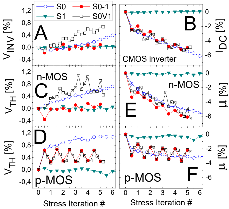
Figure 3. Relative variations of the inversion voltage (A), peak current at the inversion point (B) of the CMOS inverter, threshold voltage (C and D) and carrier mobility (E and F) of the nMOS (C and E) and pMOS (D and F), for the different sequences defined (S0, S1, S0-1 and S0V1) shown in figure 2-A.
