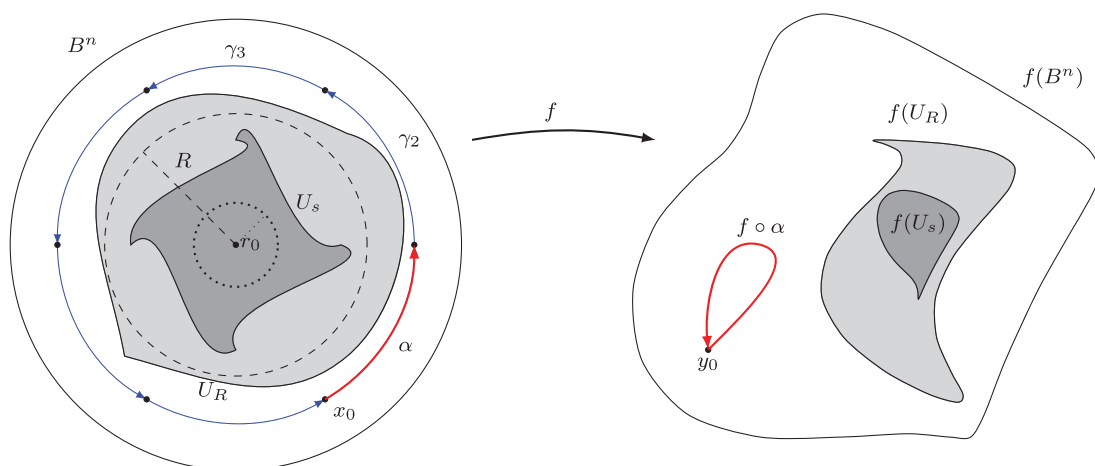
FIGURE 1 Essential objects in the proof of Proposition 4.3
