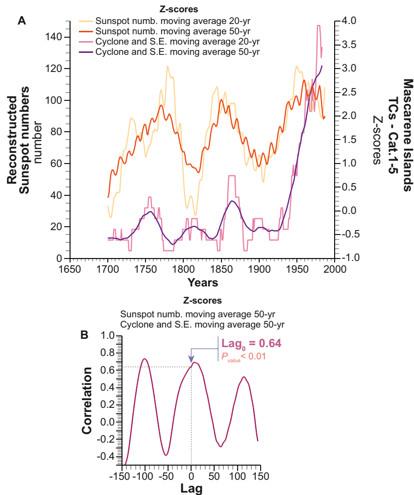
Fig. 8. A. Mascarene Islands TCs (pink = moving average 20-yr and purple = 50-yr moving average) versus reconstructed sunspot numbers (yellow = 20-yr moving average and red = 50-yr moving average). B. Cross-correlation between Mascarene Islands TCs and reconstructed sunspot numbers (50-yr moving averages). (For interpretation of the references to colour in this figure legend, the reader is referred to the web version of this article.)
