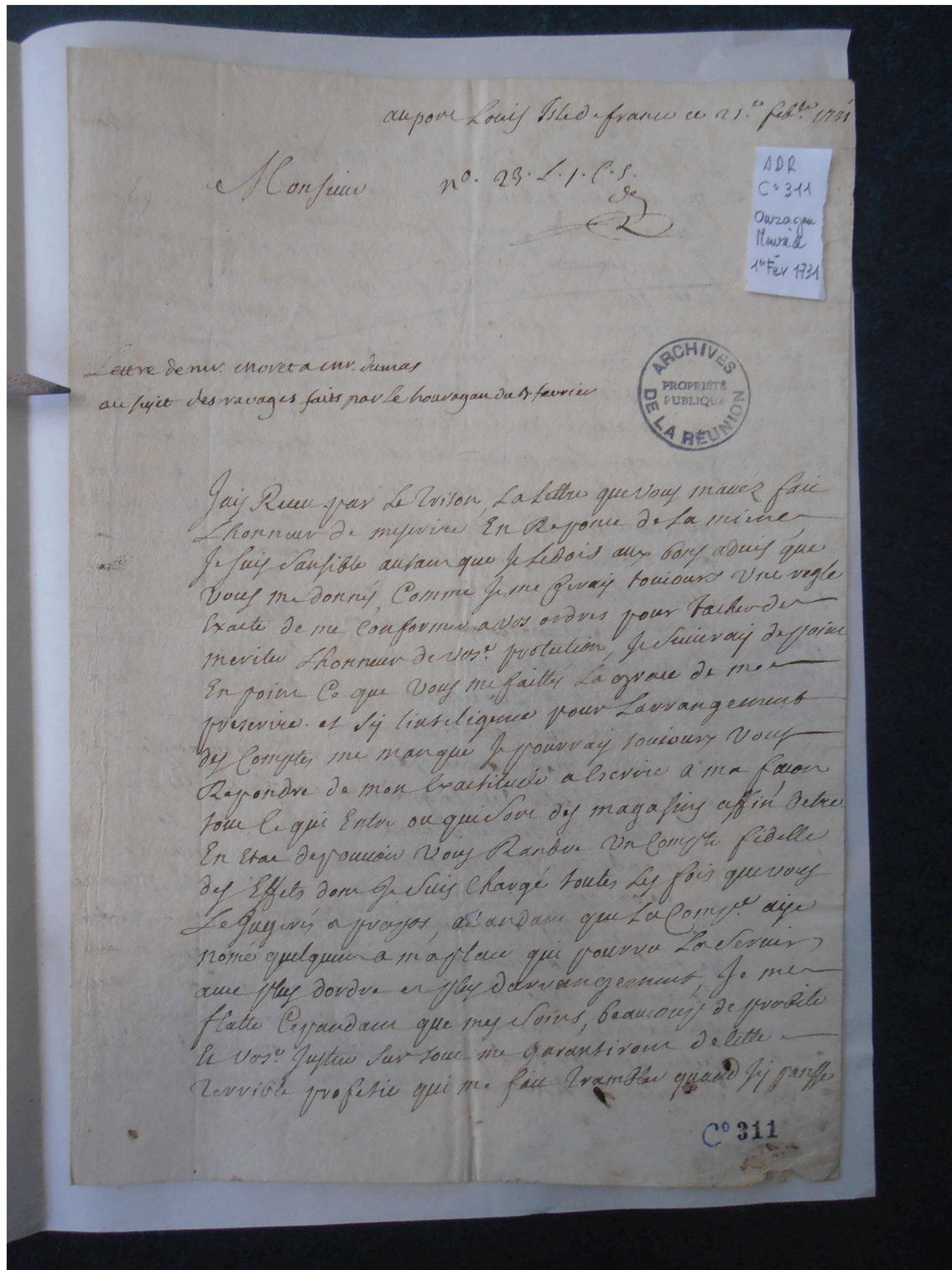
Fig. 3. Letter from the governor of Ile de France (present-day Mauritius) at Port-Louis detailing the damage caused by the TC of the 3rd February 1731. Departmental archives of La Réunion, C 311 (photograph: E Garnier).
