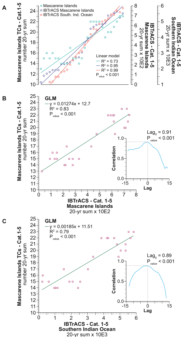
Fig. 4. A. Comparison of Mascarene Island category 1–5 TCs (green) with IBTrACS TC data for the Southern Indian Ocean and IBTrACS (red) TCs passing in proximity to the Mascarene Islands (blue; coordinates = 51 to 65 E and 15.30 to 21 S). B. Generalized Linear Model (GLM) of Mascarene Island category 1–5 TCs and IBTrACS TCs passing in proximity to the Mascarene Islands. C. GLM of Mascarene Island category 1–5 TCs and IBTrACS TC data for the Southern Indian Ocean. For the period since 1960, the two IBTrACS data series show statistically significant correlation with the historical Mascarene data ( \text{Lag}_0 = 0.91 for IBTrACS Mascarene Islands and \text{Lag}_0 = 0.89 for IBTrACS Southern Indian Ocean). (For interpretation of the references to colour in this figure legend, the reader is referred to the web version of this article.)
