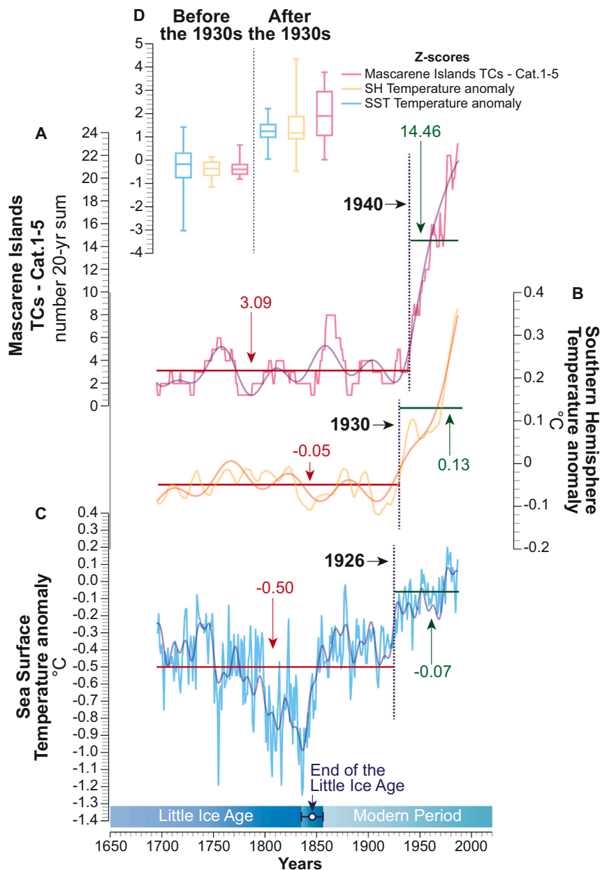
Fig. 5. A. Historical record of TC frequency (20-year moving sum) on the Mascarene Islands; B. Southern Hemisphere Temperature anomalies (Neukom et al., 2014). The anomalies are relative to the 1961–1990 temperature average; and C. Indian Ocean SST anomalies (Tierney et al., 2015). The anomalies are relative to the 1961–1990 SST average. We homogeneity tests (SNHT) on all three datasets to identify trend changes in the time series. Each discordant period is categorized by red and green lines and the mean value for each discrete period is given. D. Boxplots of all three datasets for the periods before and after the 1930s. (For interpretation of the references to colour in this figure legend, the reader is referred to the web version of this article.)
