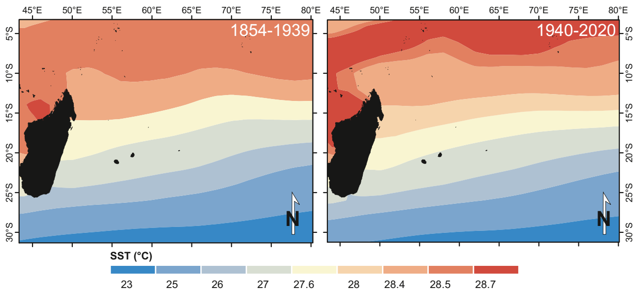
Fig. 6. Geography of SST temperatures over the SW Indian Ocean (average cyclone season SSTs) for the period 1854–1939 (A) and 1940–2020 (B). Data are from the NOAA OI SST V2 High Resolution SST Dataset and highlight the extent of ocean warming during the Great Acceleration.
