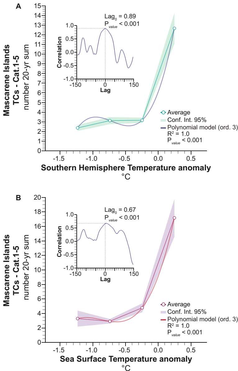
Fig. 7. TC frequency compared and contrasted with Southern Hemisphere temperature anomalies and Sea Surface Temperature anomalies. A. Number of TCs versus a gradual increase in temperature anomalies in the Southern Hemisphere. The average values are shown by blue line and dots. Each dot is associated with a confidence interval (95%). The correlation between the two time-series is highlighted by a cross-correlogram (Pvalue < 0.001). B. Number of TCs versus a gradual increase in Sea Surface Temperature anomalies. The average values are denoted by a purple line and dots. Each dot is associated with a confidence interval (95%). The correlation between the two time-series is highlighted by a cross-correlogram (Pvalue < 0.001). (For interpretation of the references to colour in this figure legend, the reader is referred to the web version of this article.)
