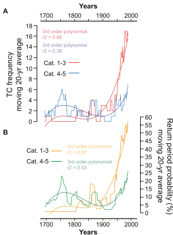
Fig. 9. A. Moving 20-year frequencies of TCs grouped into categories 1–3 (red curves) and 4–5 (blue curves). B. Smoothed (moving 20-year window) return period probabilities for category 1–3 (orange curves) and 4–5 (green curves) TCs. (For interpretation of the references to colour in this figure legend, the reader is referred to the web version of this article.)
