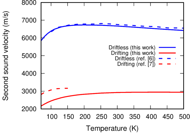
FIG. 1. Second sound drifting and driftless velocities for graphene at different temperatures from expressions (26) and (29), respectively, calculated in this work (solid lines), and from Lee et al. [7] (drifting) and Cepellotti et al. [6] (driftless) (dashed lines).
