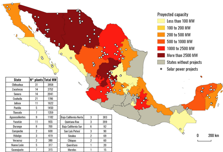
Figure 4. Solar power: operating and projected capacity per state (Mexico 2019).
