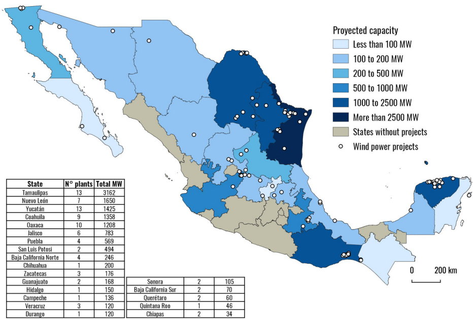
Figure 2. Wind power: operating and projected capacity per state (Mexico 2019).
