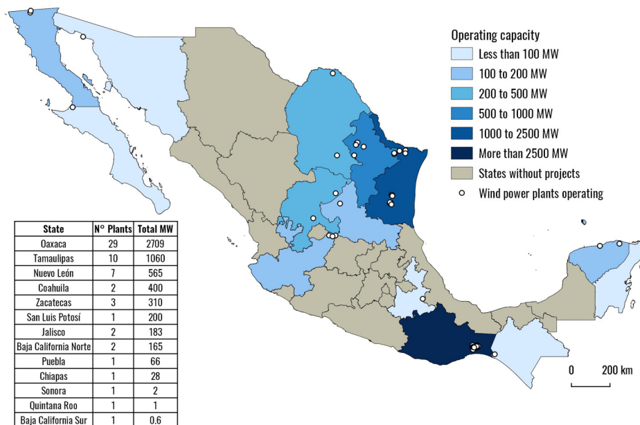
Figure 1. Wind power: operating and projected capacity per state (Mexico 2019).
