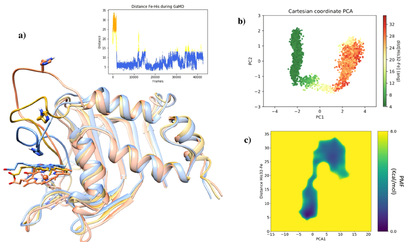
Figure 9. GaMD simulation of HasAzm with heme-Fe(III) bound. (a) Frames of GaMD showing the loop L1 closing process colored according to the distance between Fe and His32 during GaMD. Graphic of distance Fe-His32 represented. (b) Cartesian coordinate PCA analysis colored according to the distance between Fe and His32 during GaMD. (c) Reweighted PMF calculations in front of PCA1 and distance Fe-His32. (b,c) are obtained using the fragment of the trajectory in which the loop is closing.
