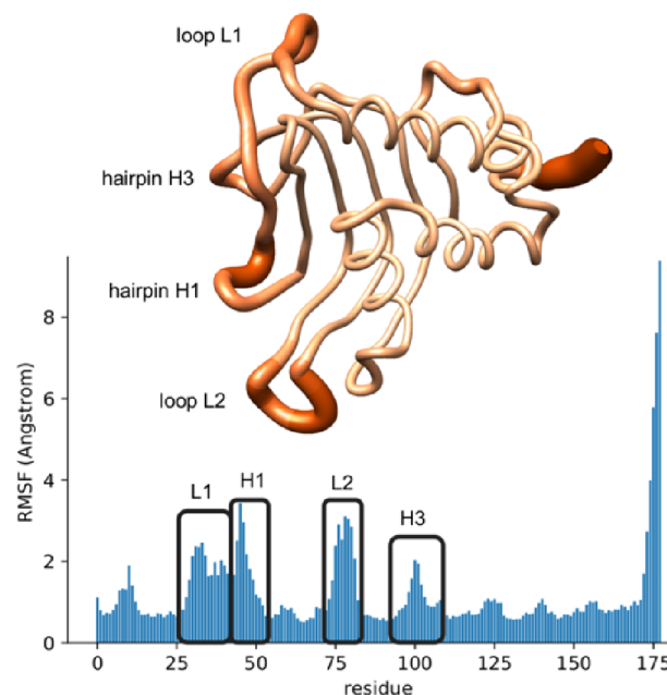
Figure 6. RMSF of apo GaMD from HasAasm with relevant regions.
