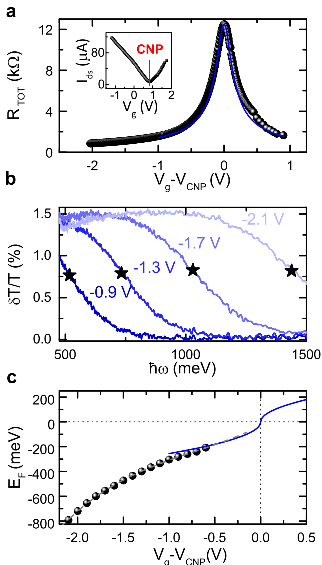
Figure 2. (a) Total resistance R_{TOT} as a function of V_g - V_{CNP} (black dots) with Drude model fitting (blue solid line) to estimate residual charge carrier density, n_0 , and gate capacitance C . Inset, I_{ds} for V_{ds} = 100 mV. (b) \delta T/T for different V_g - V_{CNP} (indicated next to the curves) as a function of photon energy \hbar\omega , showing the gate tunability of the absorption edge for interband transitions; (c) E_F determined from \delta T/T as a function of V_g - V_{CNP} (full dots) interpolated by f(x) = A_0 + A_1x + A_2x^2 + A_3x^3 with A_0 = -0.03 eV, A_1 = 0.37 eV/V, A_2 = 0.17 eV/V ^2 , A_3 = 0.08 eV/V ^3 (gray dashed line), together with the trend (blue solid line) E_F = \hbar\nu_F\sqrt{\pi n_e(V_g)} where n_e(V_g) = (V_g - V_{CNP})(C/e) is the gate-tunable charge carrier density
