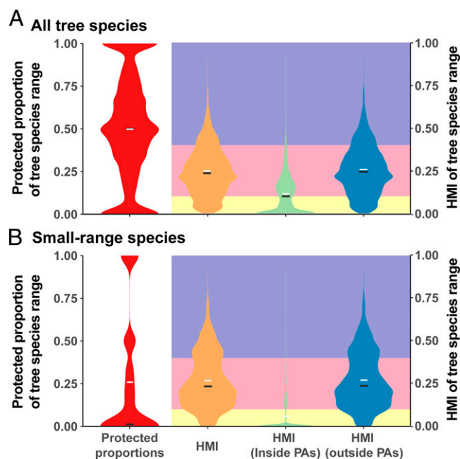
Fig. 1. Current protection status and pressures on tree species' ranges for all (A) and small-range tree species (B) (the first range size quintile). Protected proportions show the proportion of each tree species' range within existing PAs; HMI indicates the mean Human Modification Index within a tree species' range, overall, or just the range part within or outside PAs. Mean and median values are indicated by white and black solid lines in the violin density plots, respectively. Colored panes in yellow, pink, and purple, respectively, indicate low ( 0 \leq \text{HMI} \leq 0.1 ), moderate ( 0.1 < \text{HMI} \leq 0.4 ), and high to very high ( 0.4 < \text{HMI} \leq 1.0 ) levels of human modification (61). SI Appendix, Table S2 lists the mean, median, and first and third quartiles for each variable.
