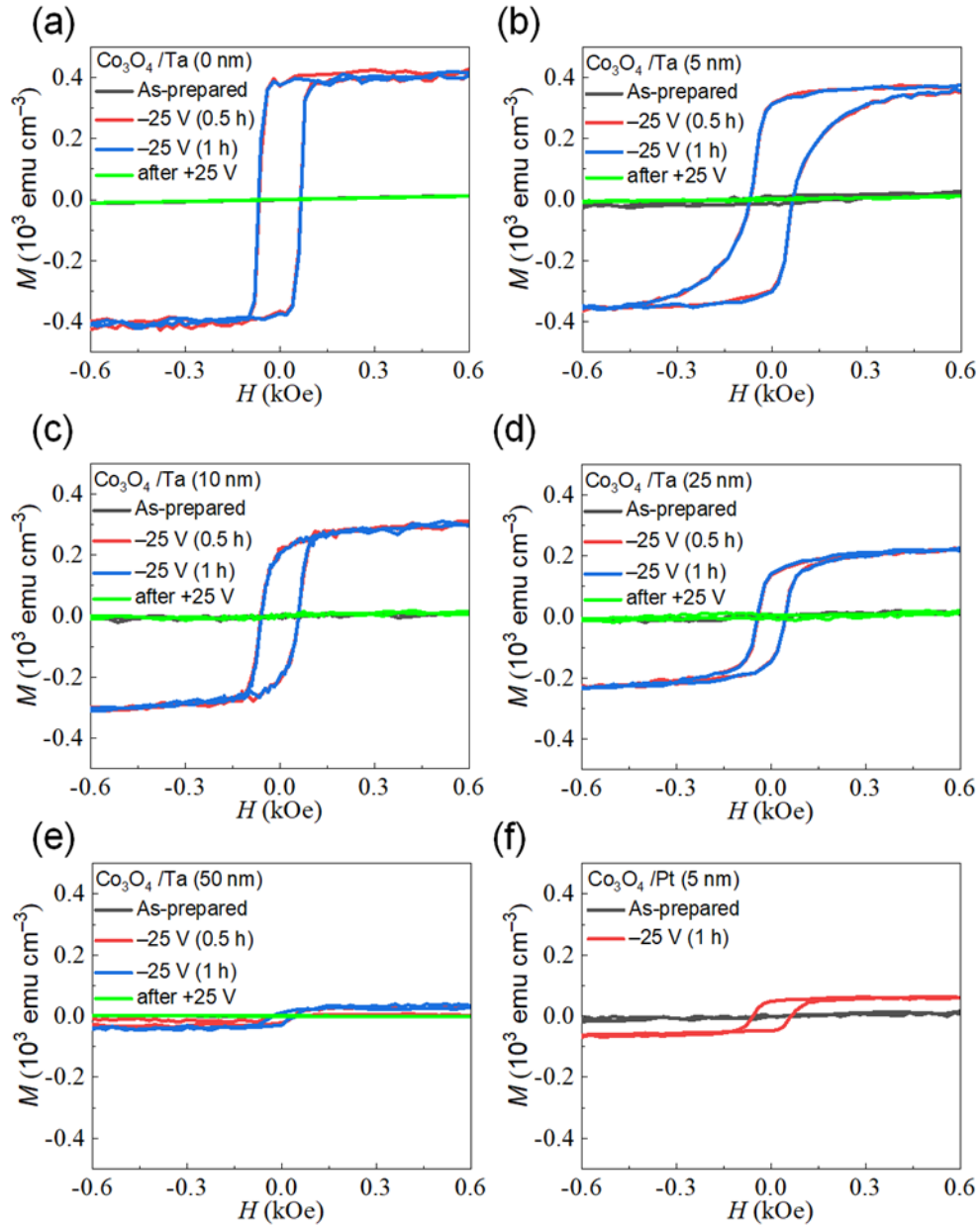
Figure 3. In-plane VSM hysteresis loops (each lasting 30 min) of the as-prepared \text{Co}_3\text{O}_4/\text{Ta} films (black), the films biased under -25 V (for 30 min in red, and for 1h in blue), and subsequently
