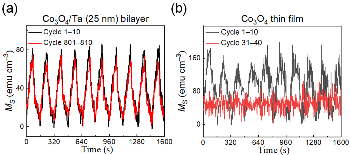
Figure 4. Magneto-ionic cyclability of (a) Co_3O_4/Ta (25 nm) bilayer films and (b) the Co_3O_4 thin films subjected to -25\ V / +25\ V voltage pulses applied with a periodicity of 80 s.
