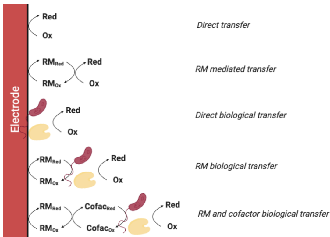
Figure 3. Schematic representation of different mechanisms of electron transfer from electrode to redox species.
