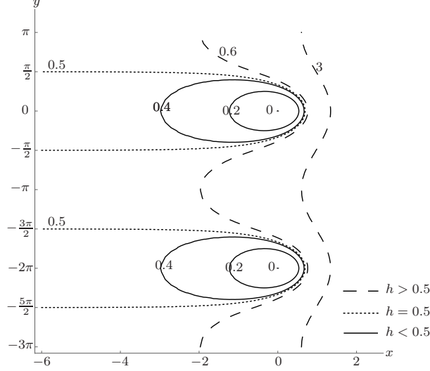
FIGURE 2. The level sets of H_f .
