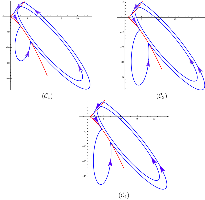
FIGURE 4. The two limit cycles of the discontinuous piecewise linear differential system (C_1) for (2)–(3), (C_3) for (5)–(6) and (C_4) for (7)–(8).
