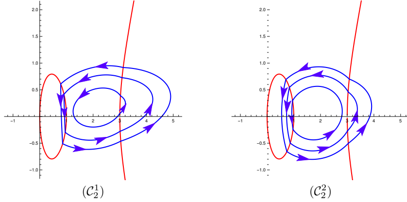
FIGURE 14. The three limit cycles of the discontinuous piecewise linear differential system (\mathcal{C}_2^1) for (60)–(62), and (\mathcal{C}_2^2) for (64)–(66).
