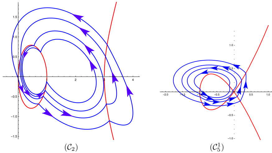
FIGURE 19. The four limit cycles of the discontinuous piecewise linear differential system (\mathcal{C}_2) for (92)–(94), and (\mathcal{C}_5^1) for (96)–(98).
