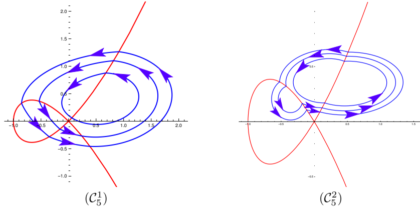
FIGURE 15. The three limit cycles of the discontinuous piecewise linear differential system (\mathcal{C}_5^1) for (68)–(70), and (\mathcal{C}_5^2) for (71)–(73).
