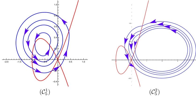
FIGURE 18. The four limit cycles of the discontinuous piecewise linear differential system (\mathcal{C}_5^1) for (86)–(88), and (\mathcal{C}_5^2) for (89)–(91).
