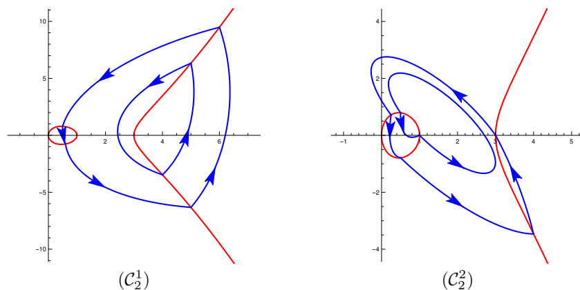
FIGURE 8. The two limit cycles of the discontinuous piecewise linear differential system (\mathcal{C}_2^1) for (22)–(24), and (\mathcal{C}_2^2) for (26)–(28).
