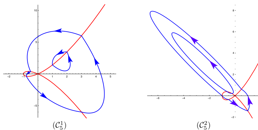
FIGURE 9. The two limit cycles of the discontinuous piecewise linear differential system (\mathcal{C}_5^1) for (30)–(32), and (\mathcal{C}_5^2) for (33)–(35).
