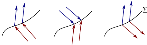
FIGURE 3. Crossing, sliding and escaping regions, respectively.
