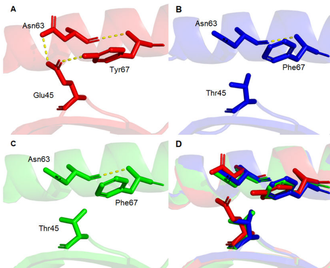
Figure 5: A-C. Representation of residues 45, 63 and 67 in HLA-B*07:02, -B*35:01 and -B*51:01. HLA in HLA-B*07:02 (A), -B*35:01 (B) and -B*51:01 (C). D. Superposition of HLA-B*07:02 (red), -B*35:01 (blue) and B*51:01 (green). Residues 46, 63 and 67 are represented as sticks. Polar contacts are represented as dotted yellow lines. PDB entries: 1E27, 1A1N and 6UJ7.
