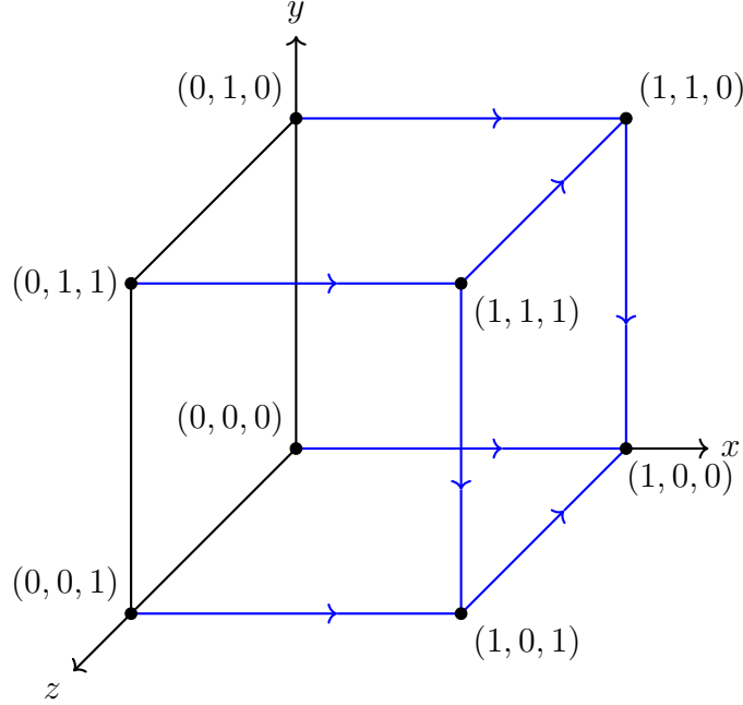
Figure 5: \preceq^{f,(1,1,1)}
