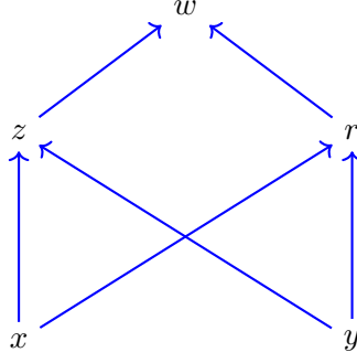
Figure 3: \succeq_0
