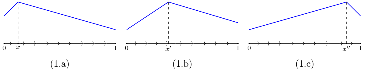
Figure 1: Single-peaked preferences
