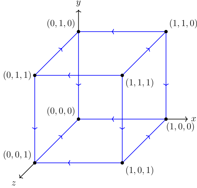
Figure 9: Path representation of P_i^{(1,1,1)}
