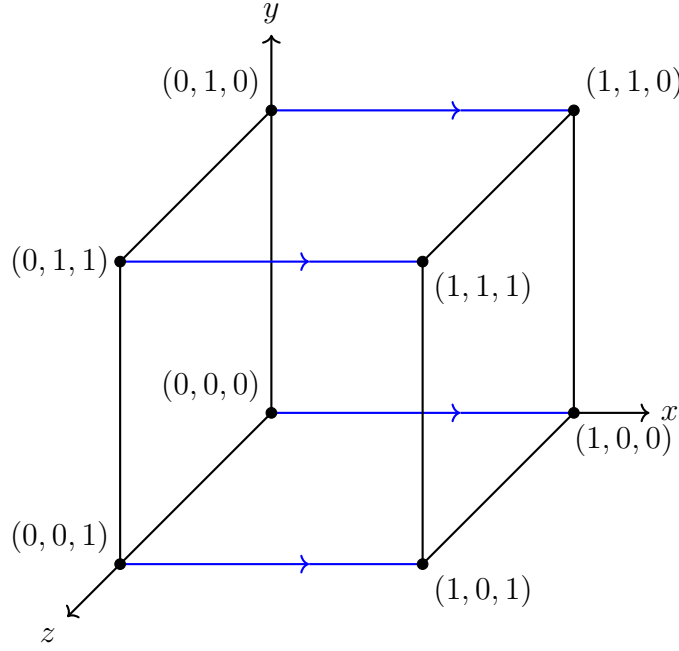
Figure 4: \succeq_0
