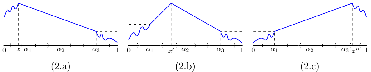
Figure 2: Local and weakly single-peaked preferences
