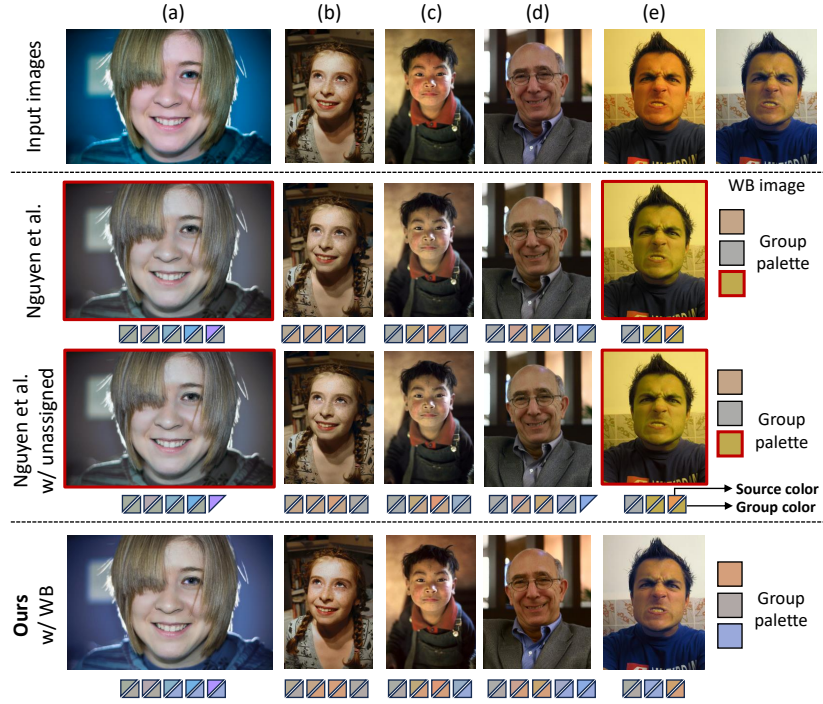
Figure 5: Results after applying the white-balance correction module are presented in the following order: input images, results from two versions by Nguyen et al. , and our results. In the images, red boxes are used to highlight unsatisfactory recolored images and palette colors. We obtain better color consistency among the recolored images by incorporating the white balance correction. The images used for this demonstration were sourced from Flickr [Fli04].
