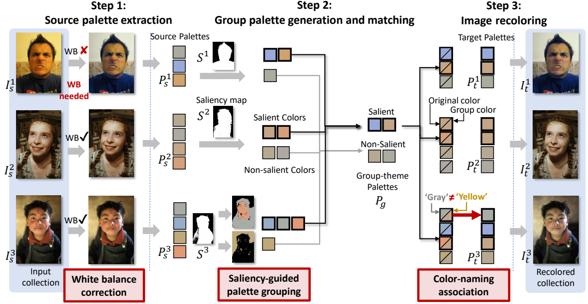
Figure 2: Our image collection recoloring framework. Given the input collection of images, I_s^i . Step 1: the source palette P_s^i of each image I_s^i is extracted by k-means clustering. White-balance correction (either automatic or manual) is applied before the clustering procedure. Step 2: Colors in each source palette P_s^i are categorized based on the saliency map S^i into two groups: a sub-palette for the salient regions, and a sub-palette for the non-salient regions. The group palette P_g is computed based on the salient and non-salient source palettes of all the input images, respectively. The colors in each source palette match the color in the group palette. Color associations between the source and the group palette with inconsistent color names are removed. Step 3: The images are recolored based on the mapping between source palette P_s^i and group palette P_g .
