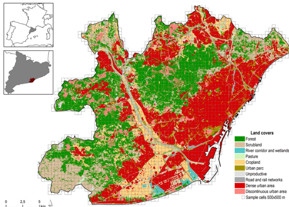
Fig. 1. Major land covers in the Barcelona Metropolitan Area (BMA).
