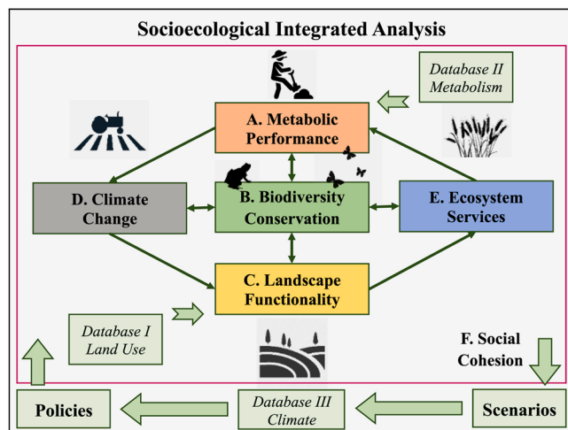
Fig. 3. Socioecological Integrated Analysis (SIA) of the metropolitan green infrastructure of Barcelona, considering six interrelated dimensions.
