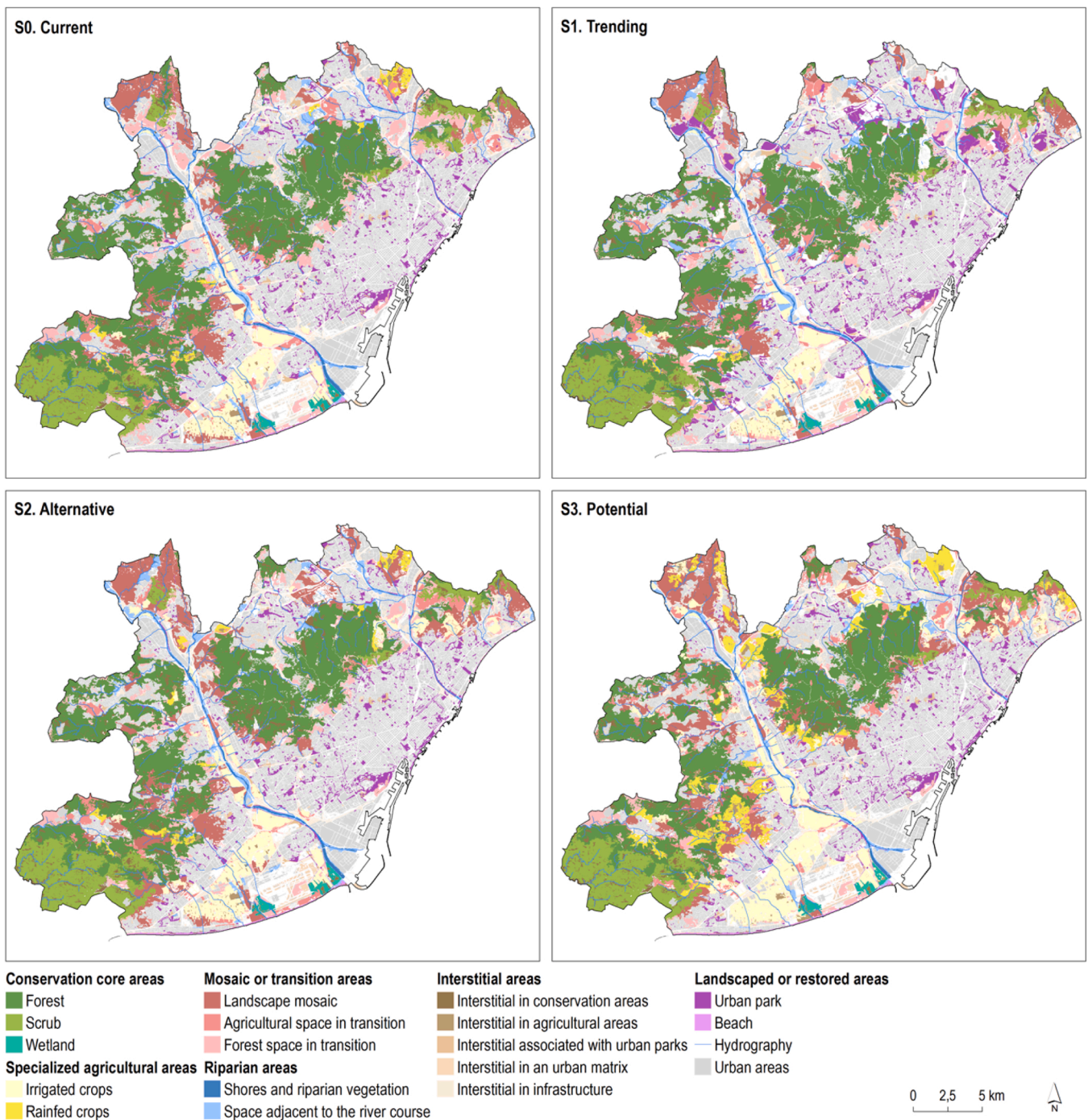
Fig. 4. Structural delimitation of the green infrastructure of the Barcelona Metropolitan Area (BMA) for the S0 Current , S1 Trending , S2 Alternative , and S3 Potential scenarios.
