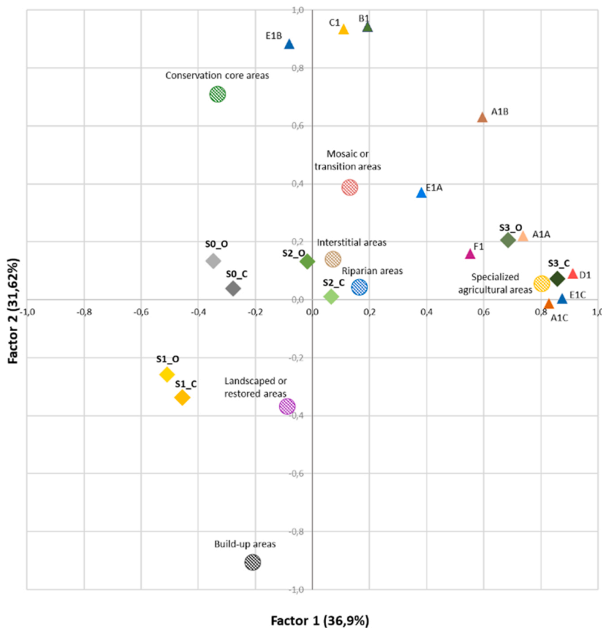
Fig. 5. Exploratory Factor Analysis (EFA) of the Barcelona Metropolitan Area (BMA) green infrastructure. Open space categories (circles), SIA indicators* (triangles), and land planning and agricultural management scenarios (rhombi) * * are displayed.
