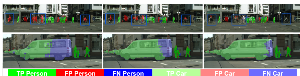
Figure 4. Analogous to Figure 3 for the classes Person and Car.
